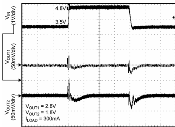
Line Transient
