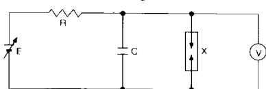
測定回路 Measuring Circuit
