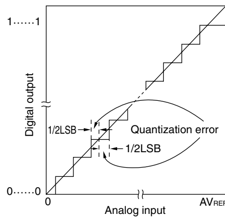
Figure 10-15. Quantization Error
