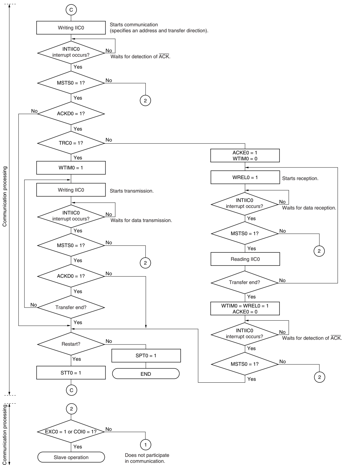
Figure 14-24. Master Operation in Multi-Master System (3/3)
