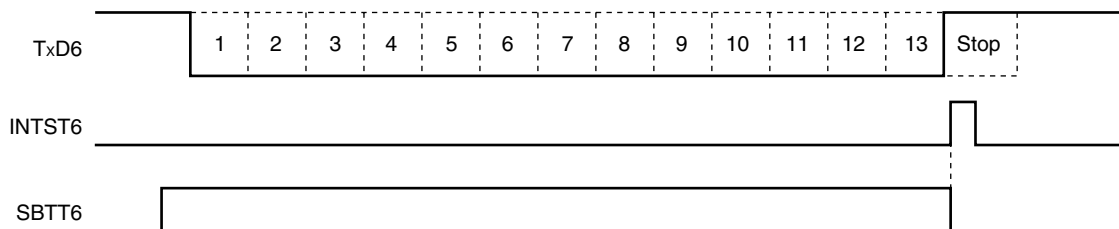
Figure 12-22. SBF Transmission
