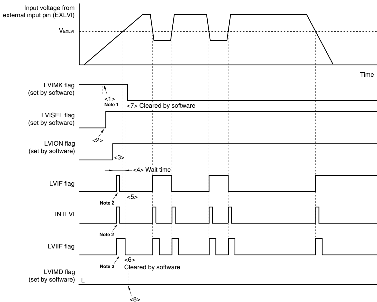
Figure 19-8. Timing of Low-Voltage Detector Interrupt Signal Generation (Detects Level of Input Voltage from External Input Pin (EXLVI))
