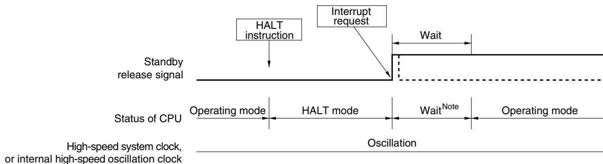
Figure 16-3. HALT Mode Release by Interrupt Request Generation
