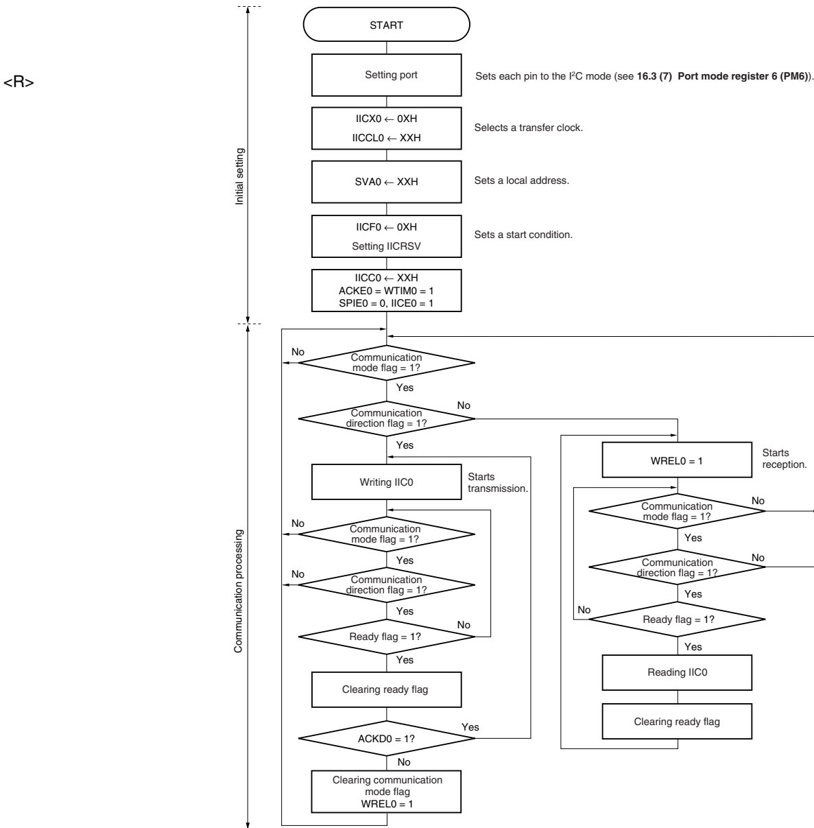
Figure 14-25. Slave Operation Flowchart (1)
