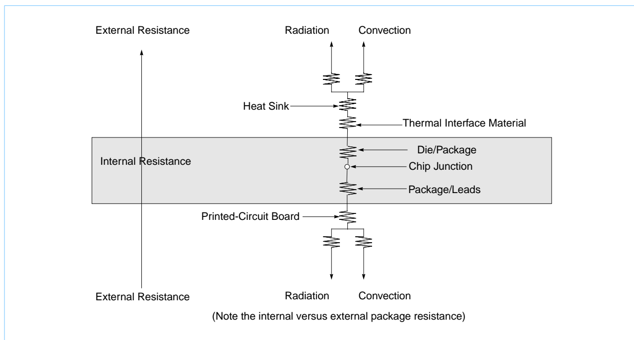
Figure 25. C4 Package with Heat Sink Mounted to a Printed-Circuit Board
