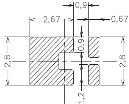
Soldering patterns
