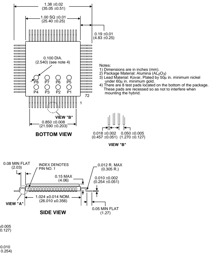
FIGURE 4. BU-65178G / 65179G* /61588G /61688G*/61689G* MECHANICAL OUTLINE (GULL LEAD)
