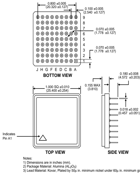
FIGURE 3. BU-65178P / 65179P* /61588P /61688P*/61689P* MECHANICAL OUTLINE (PIN GRID ARRAY - PGA)
