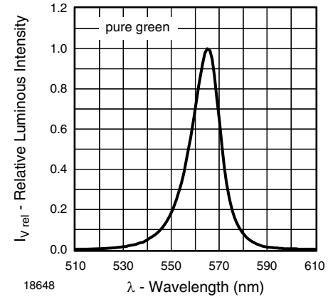
Figure 5. Relative Luminous Intensity vs. Wavelength
