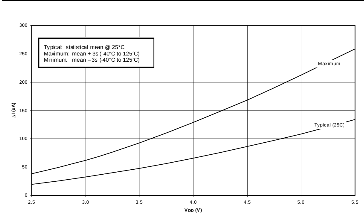
FIGURE 21-14: TYPICAL AND MAXIMUM \Delta I_{RPU} vs. V_{DD} (MEASURED PER INPUT PIN, -40^{\circ}\text{C} TO +125^{\circ}\text{C} )
