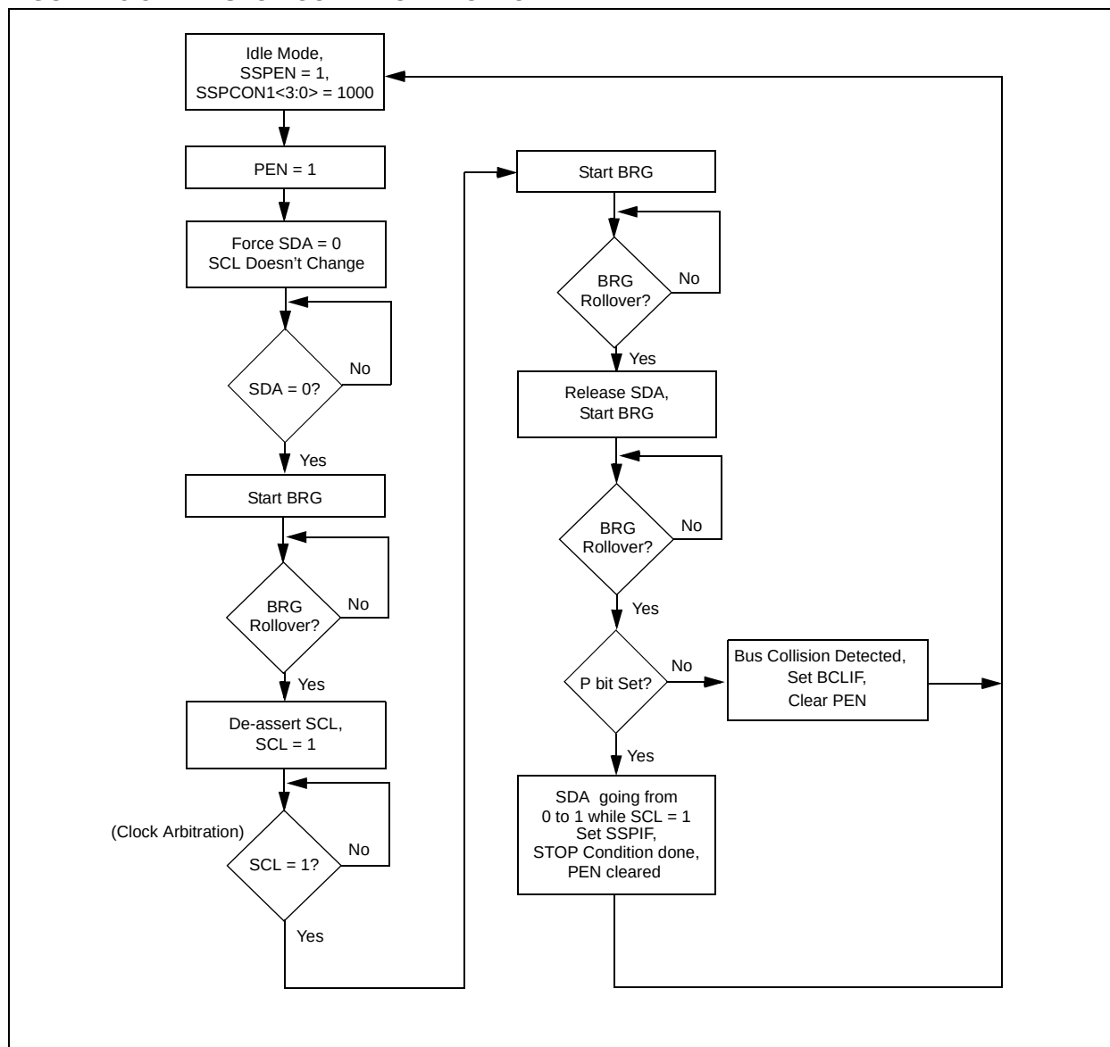
FIGURE 15-32: STOP CONDITION FLOW CHART
