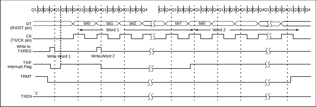
FIGURE 14-8: SYNCHRONOUS TRANSMISSION
