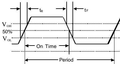
Figure 1. Output Waveform
