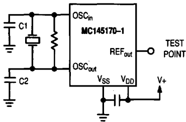
Figure 9. Test Circuit
