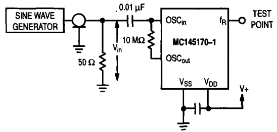
Figure 8. Test Circuit
