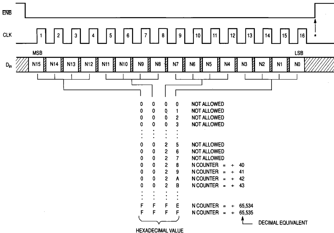
Figure 16. N Register Access and Format (16 Clock Cycles Are Used)
