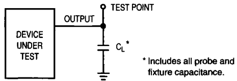
Figure 12. Test Circuit
