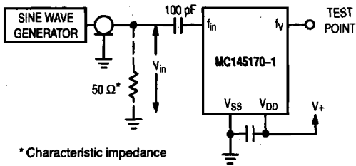
Figure 7. Test Circuit
