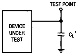
Figure 5. Test Circuit
