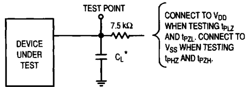
Figure 6. Test Circuit
