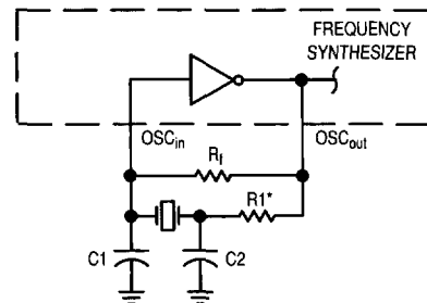
Figure 18. Pierce Crystal Oscillator Circuit
