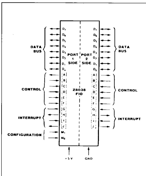
Figure 1 : FIO Logic Functions.
