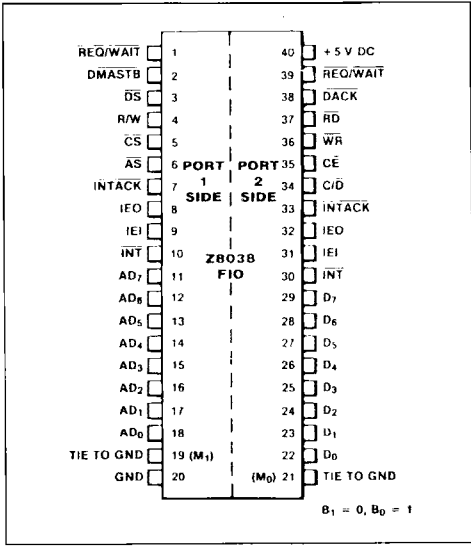
Figure 57 : Z-BUS-Low-Byte to Non-Z-BUS.
