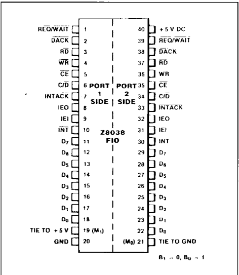
Figure 65 : Non-Z-BUS to Non-Z-BUS.
