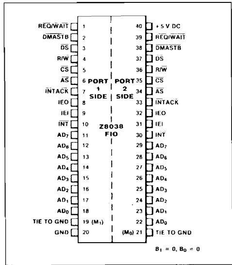
Figure 56 : Z-BUS-Low-Byte to Z-BUS-Low-Byte.
