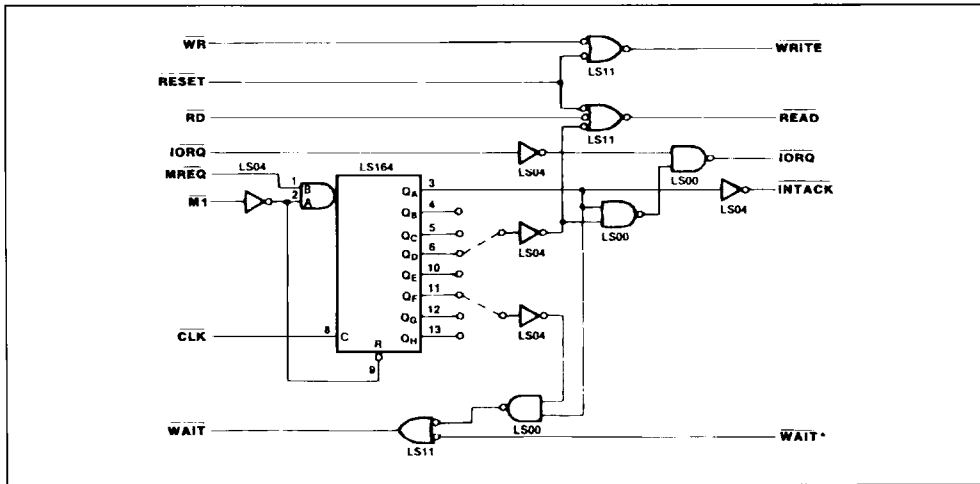
Figure 53 : Z80 \overline{\text{INTACK}} Generation for the FIO.
