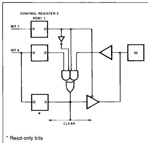
Figure 39 : CLEAR : CPU-to-I/O Operation.
