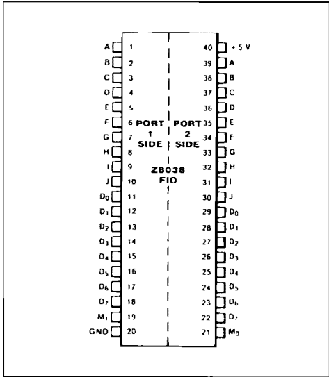
Figure 2 : Dual in Line Pin Connection.
