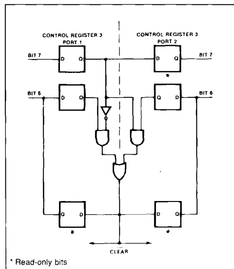
Figure 37 : CLEAR : CPU-to-CPU Operation.
