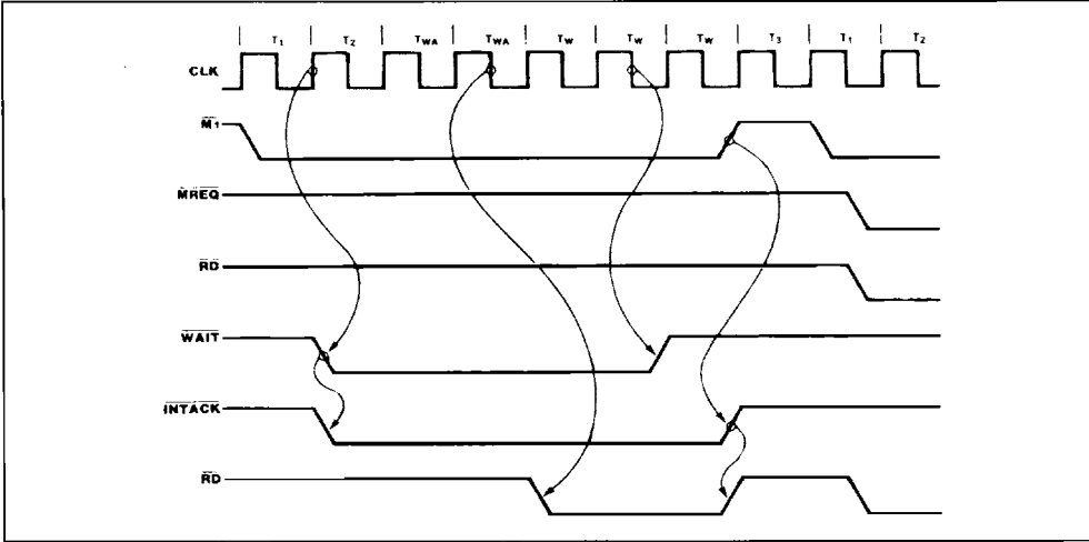
Figure 53 : Z80 \overline{\text{INTACK}} Generation for the FIO.
