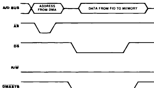
Figure 25 : Z-BUS FIO-to-Memory Data Transactions.
