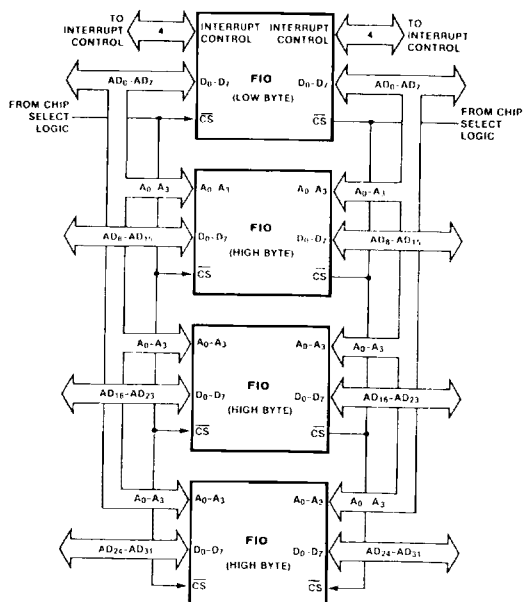
Figure 4 : FIO 32-Bit Width Expansion.
