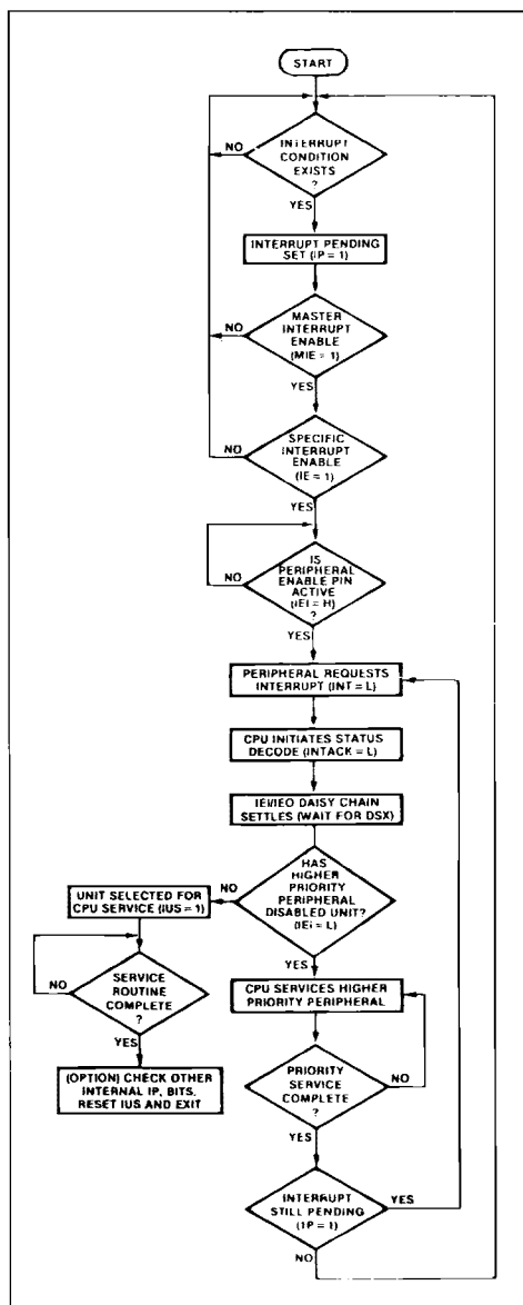
Figure 31 : Interrupt Flowchart.
