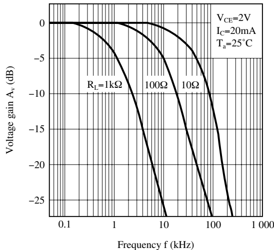
Fig.14 Frequency Response
