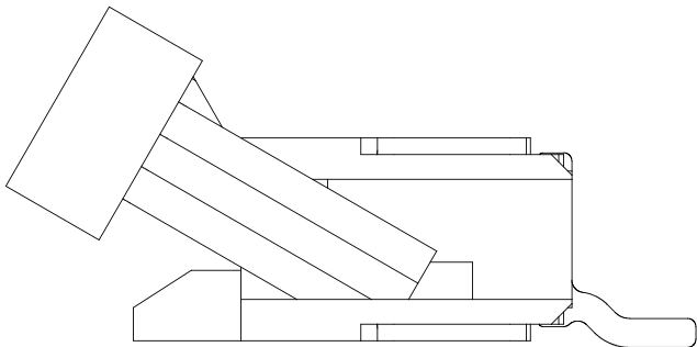
-01 LEAD STYLE [CONTACT BOTTOM] (WITH CAM OPEN)
