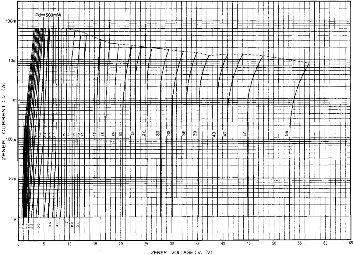
Fig. 1 Zener characteristic
