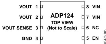
Figure 3. ADP124 Fixed Output MSOP Pin Configuration
