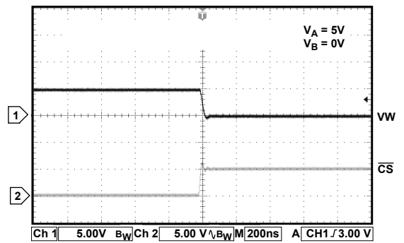
Figure 26. Midscale Glitch, Code 0x80 to 0x7F
