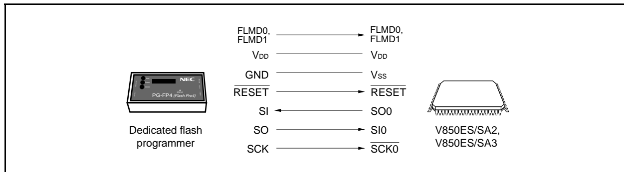
Figure 21-5. Communication with Dedicated Flash Programmer (CSI0)
