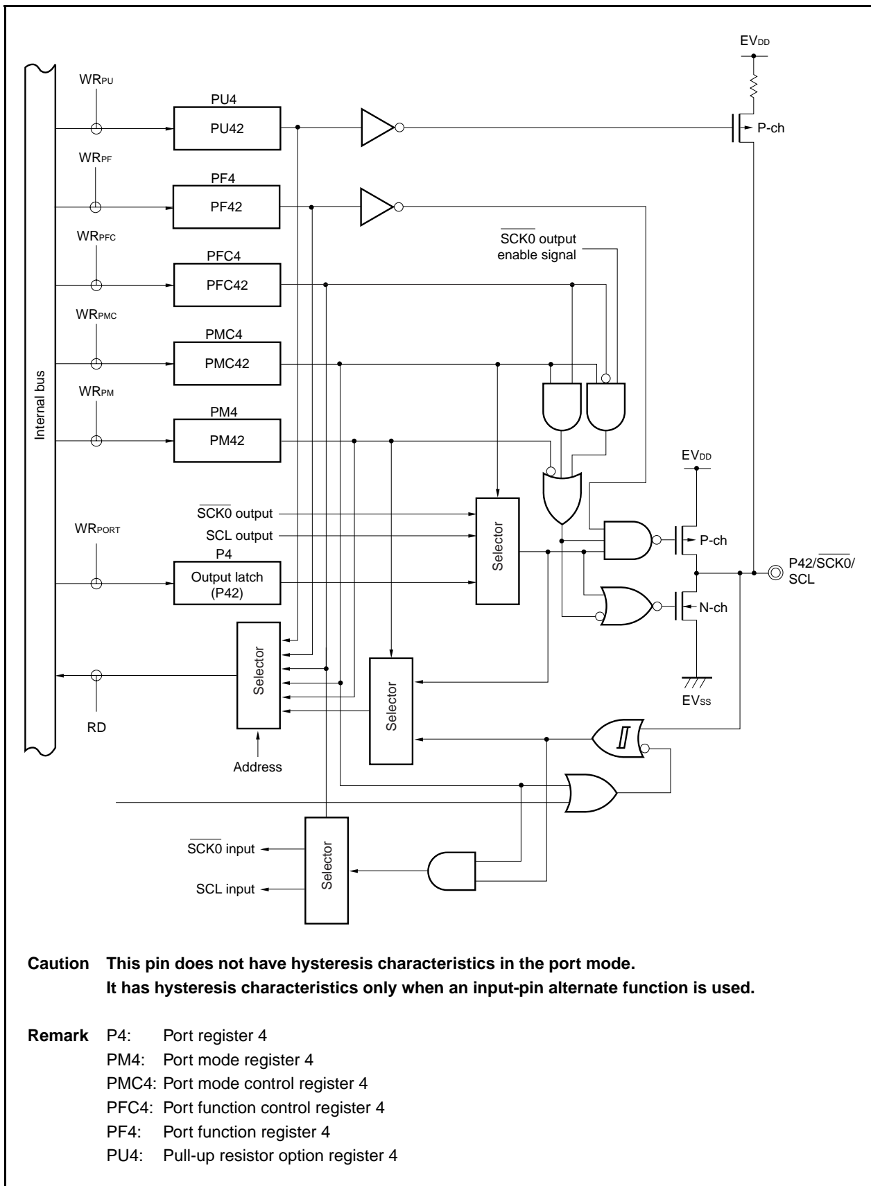
Figure 4-13. Block Diagram of P42
