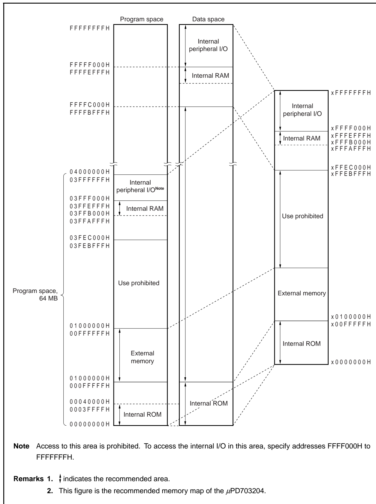
Figure 3-11. Recommended Memory Map
