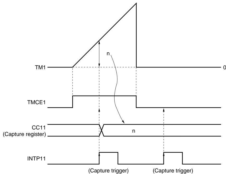
Figure 7-4. Capture Operation Example (TM1)
