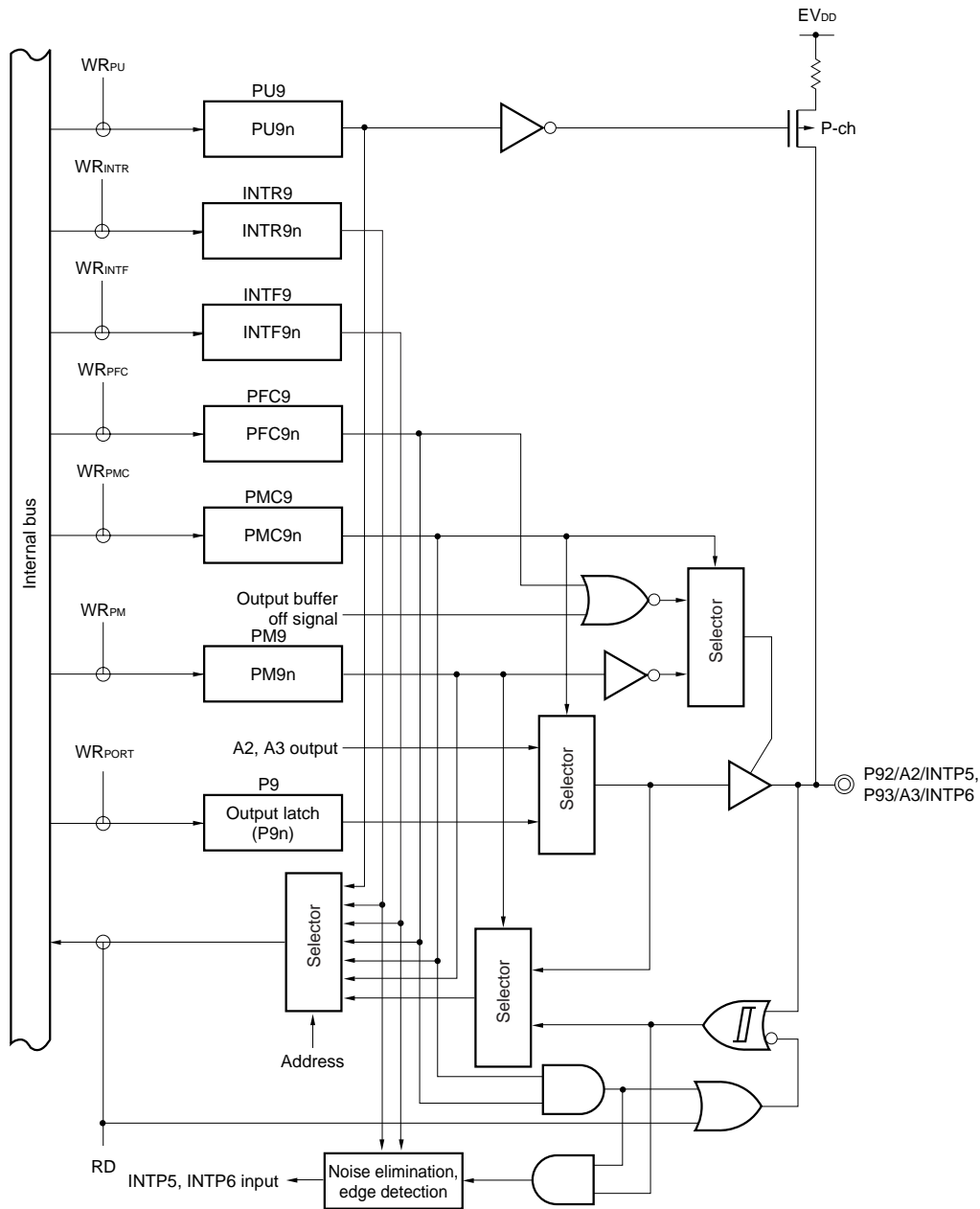
Figure 4-19. Block Diagram of P92 and P93
