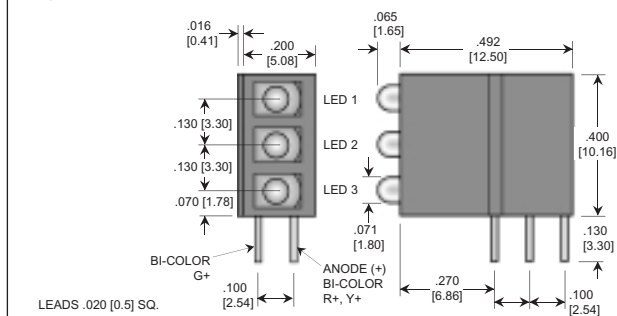
Figure 1. Tri-Level Indicator LEDs
