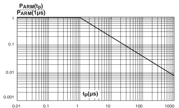
Fig. 2: Normalized avalanche power derating versus pulse duration.
