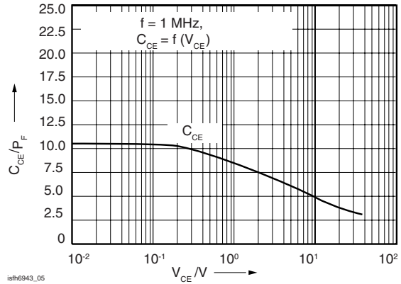
Figure 5. Transistor Capacitances (typ.)
