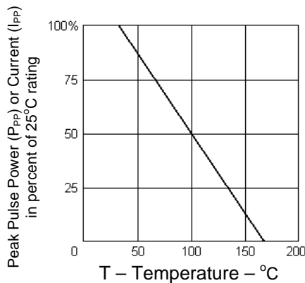
FIGURE 3 DERATING CURVE
