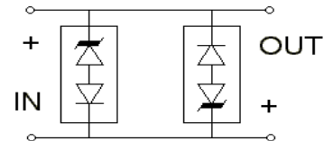
FIGURE 6 Optional Bidirectional configuration (two TVS devices in anti-parallel)
