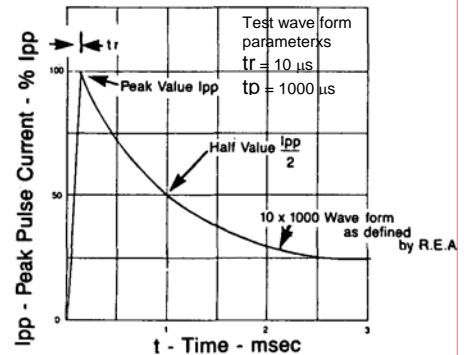
FIGURE 2 PULSE WAVEFORM
