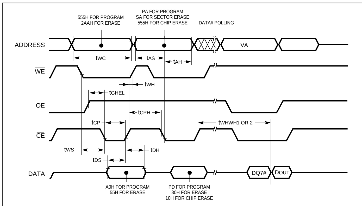
Figure 17. AC Waveform:
