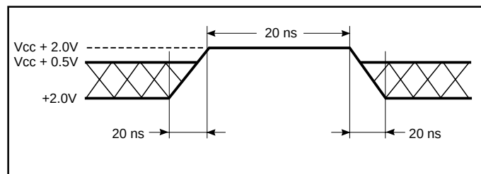
Figure 10. Maximum Positive Overshoot Waveform
