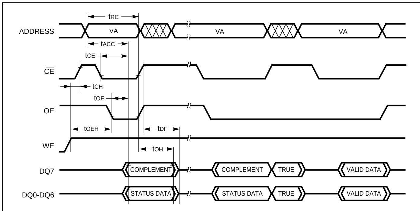
Figure 15. AC Waveform:
