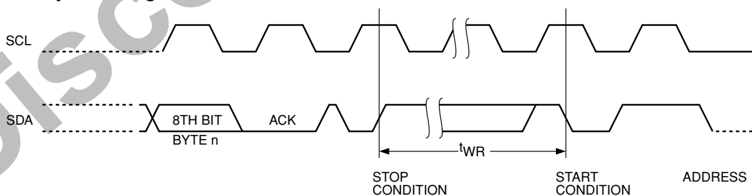
Figure 3. Start/Stop Timing
