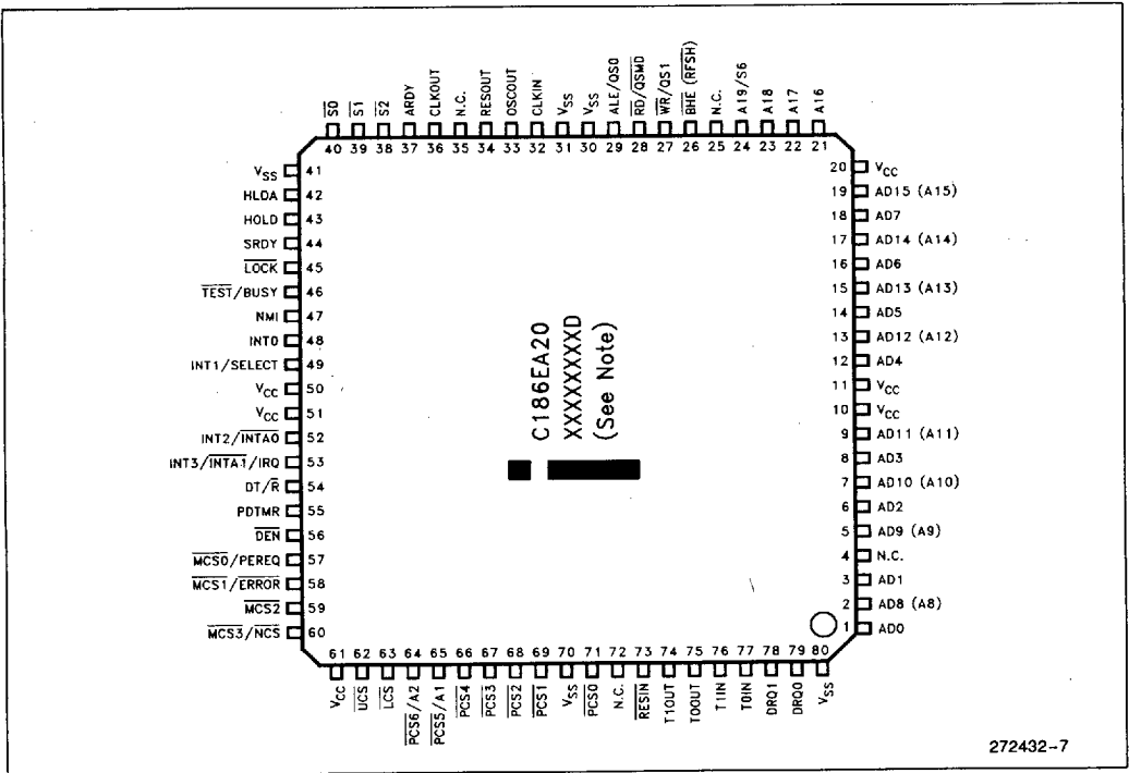
Figure 7. Shrink Quad Flat Pack (SQFP) Pinout Diagram
