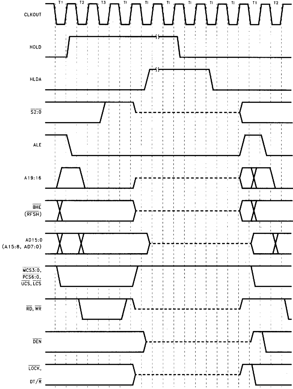
Figure 21. HOLD/HLDA Waveform
