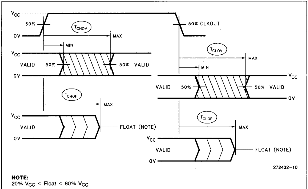
Figure 10. Output Delay and Float Waveform
