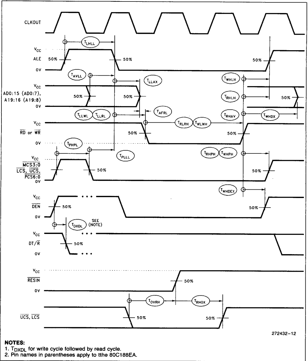
Figure 12. Relative Signal Waveform
