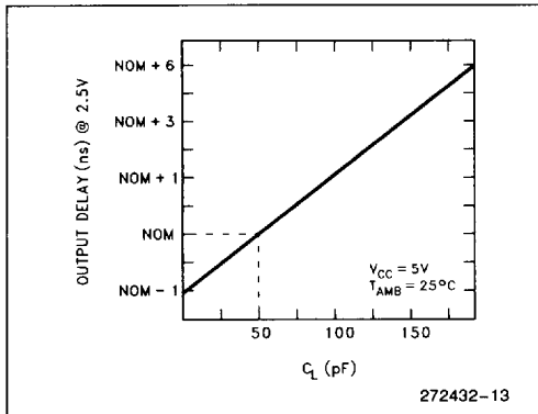
Figure 13. Typical Output Delay Variations Versus Load Capacitance
