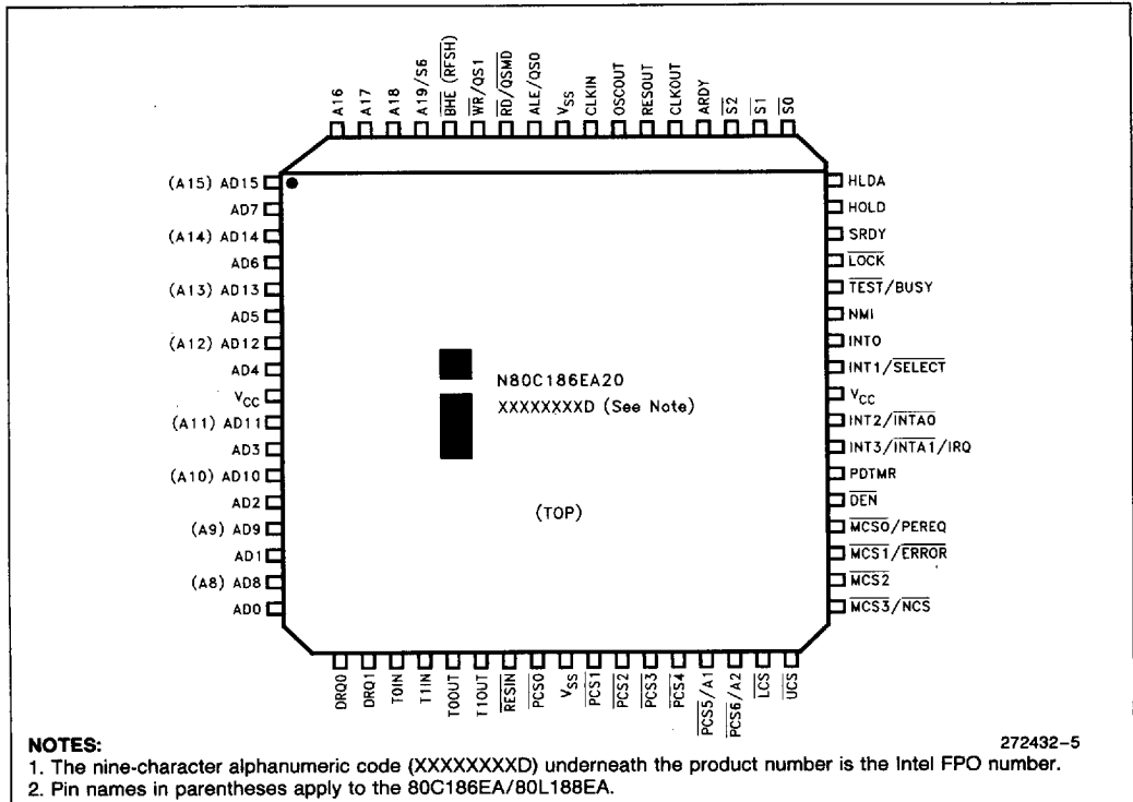
Figure 5. 68-Lead PLCC Pinout Diagram
