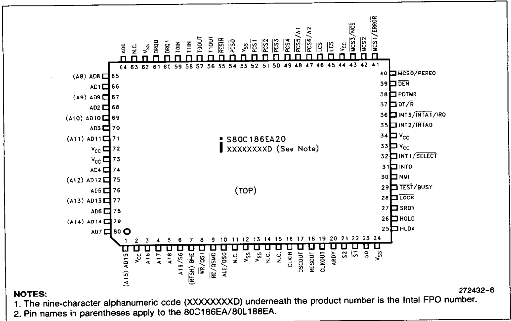
Figure 6. Quad Flat Pack (EIAJ) Pinout Diagram
