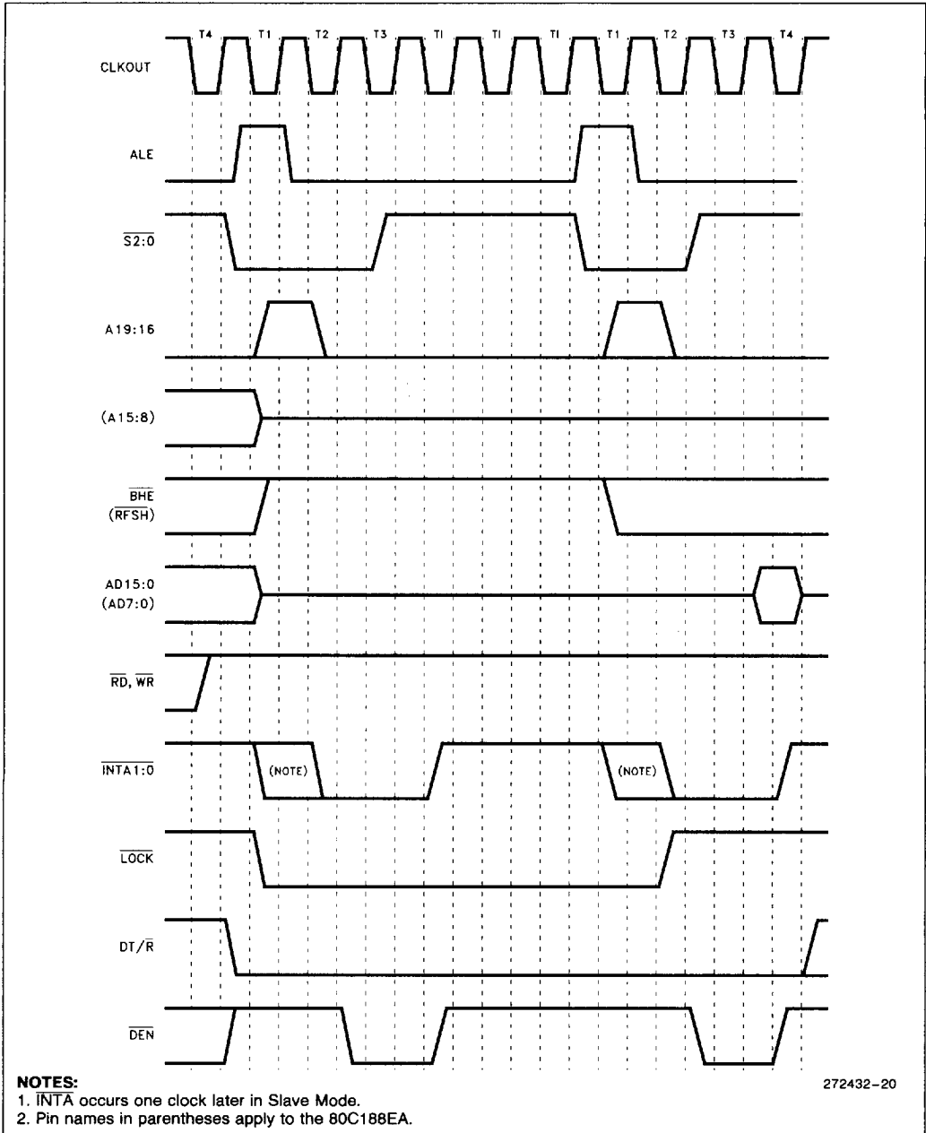
Figure 20. INTA Cycle Waveform
