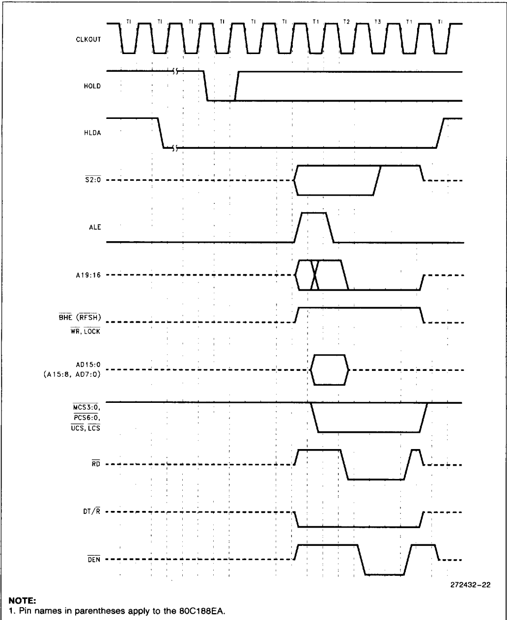
Figure 22. DRAM Refresh Cycle During Hold Acknowledge
