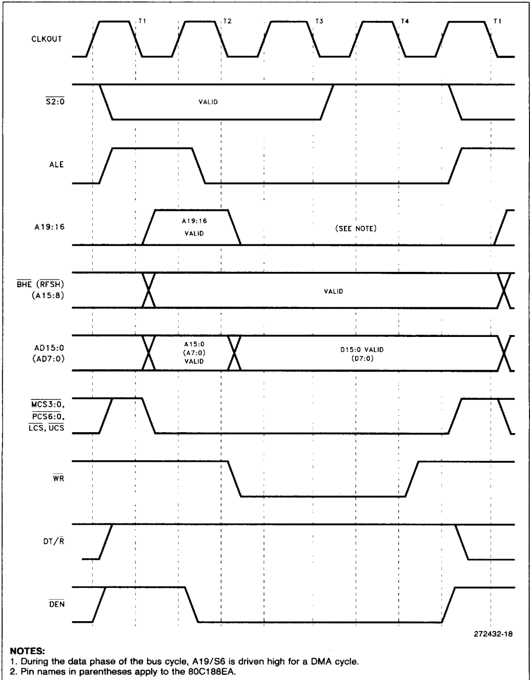
Figure 18. Write Cycle Waveform
