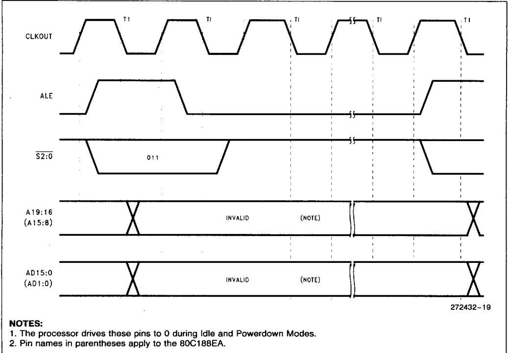
Figure 19. Halt Cycle Waveform
