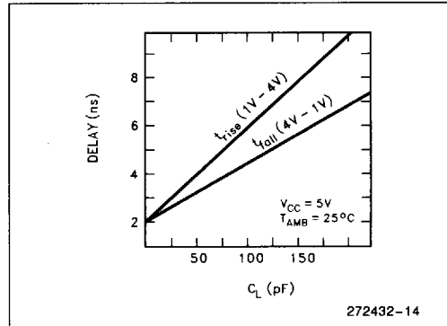
Figure 14. Typical Rise and Fall Variations Versus Load Capacitance
