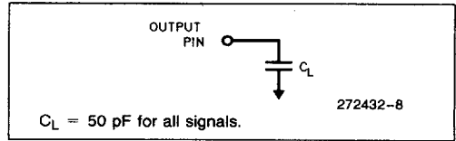
Figure 8. AC Test Load
