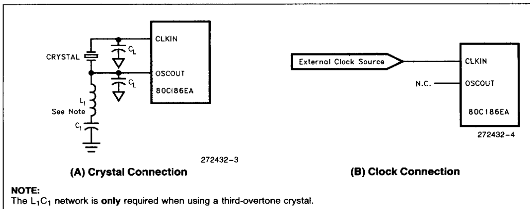
Figure 2. Clock Configurations
