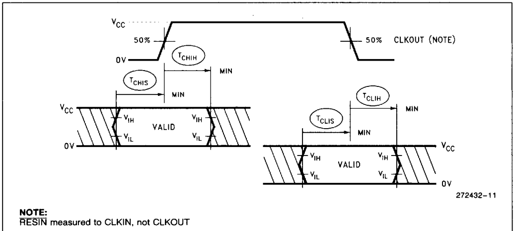
Figure 11. Input Setup and Hold
