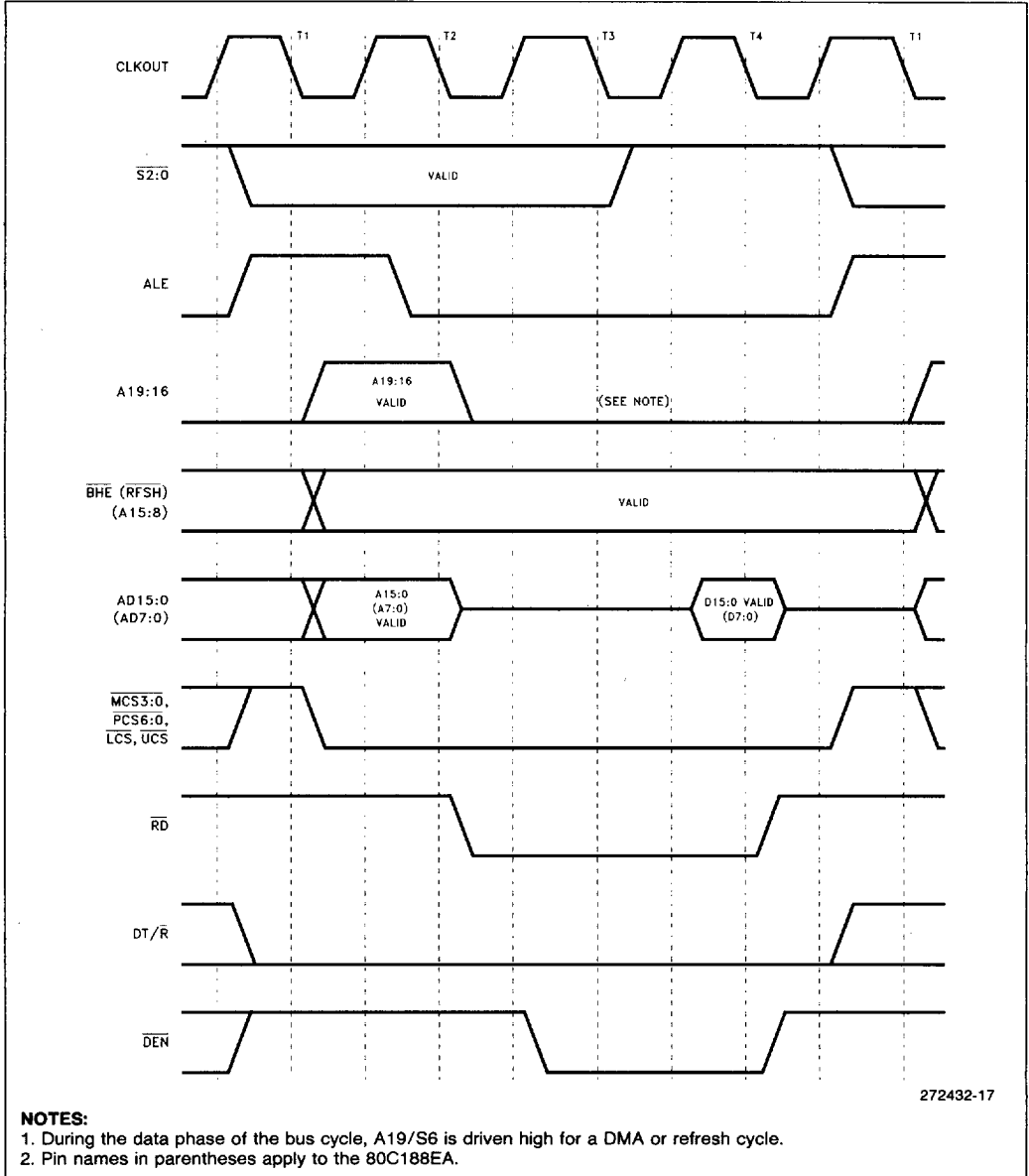
Figure 17. Read, Fetch and Refresh Cycle Waveform
