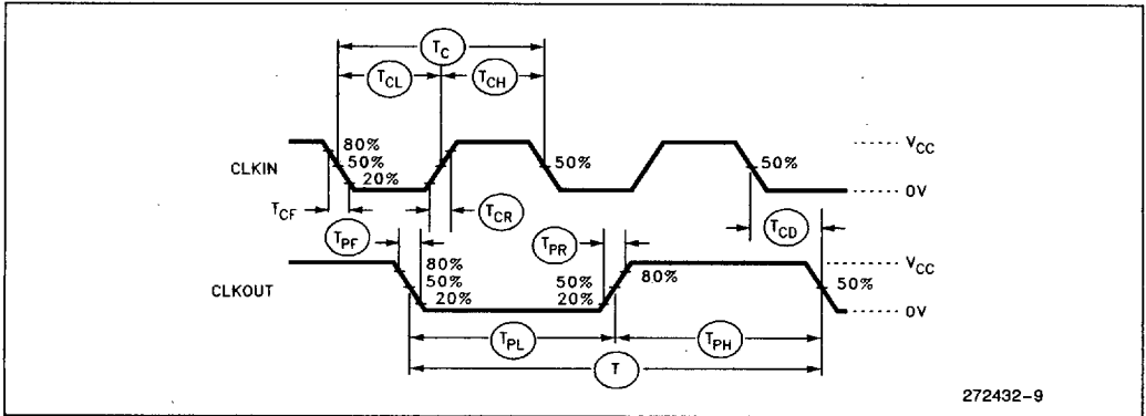
Figure 9. Input and Output Clock Waveform
