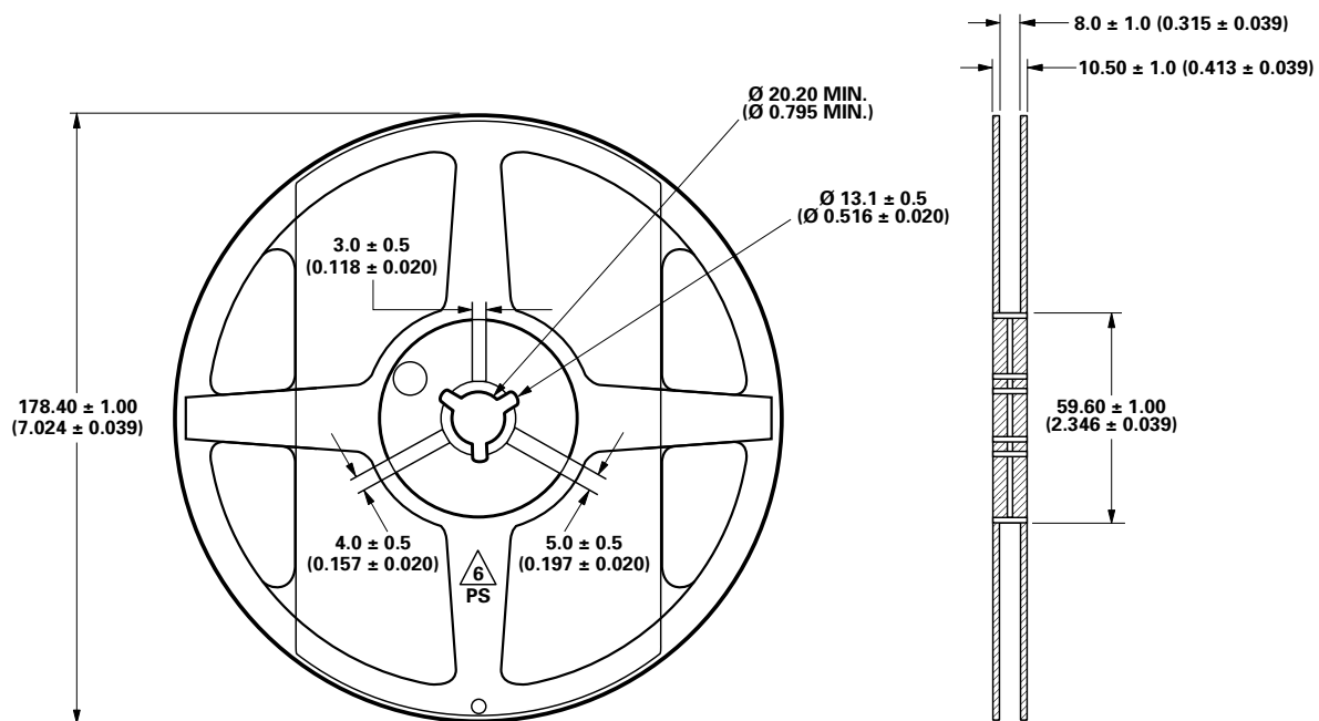
Figure 9. Reel Dimensions.
