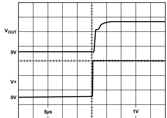
Figure 63. AD855x Output Behavior on Power-Up
