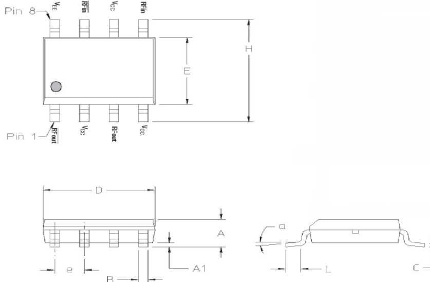
Figure 2. Package & Dimensions
