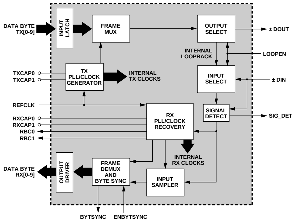
Figure 2. HDMP-16x6A/T1636A Transceiver Block Diagram.
