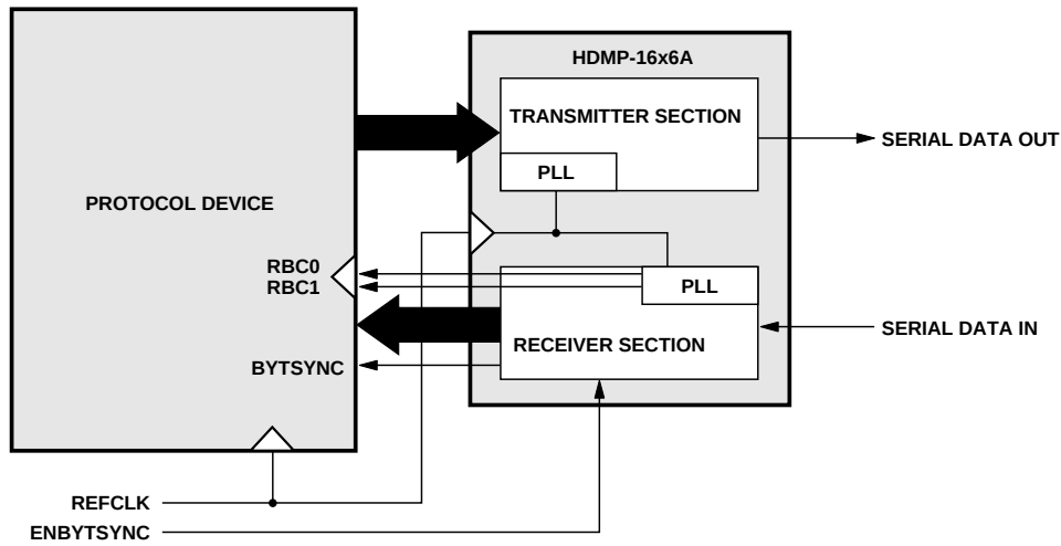
Figure 1. Typical Application Using the HDMP-16x6A/T1636A.
