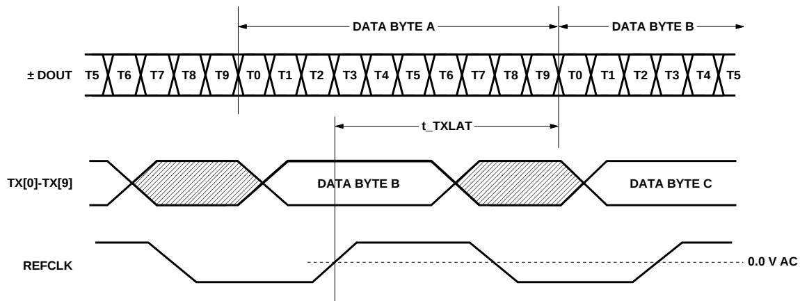
Figure 4. Transmitter Latency.
