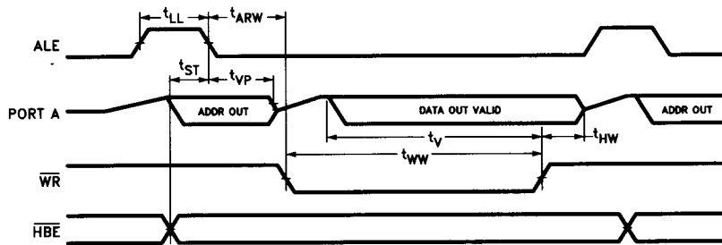
FIGURE 4. Write Cycle
