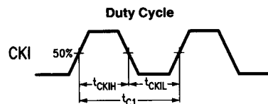
FIGURE 1. CKI Input Signal
