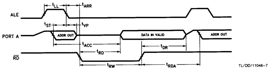
FIGURE 5. Read Cycle
