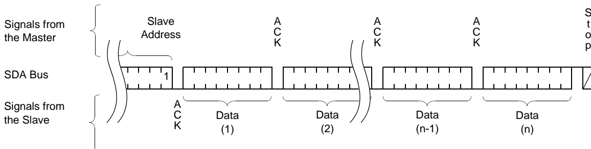
Figure 14. Sequential Read Sequence
