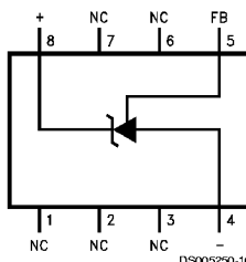
SO Package
