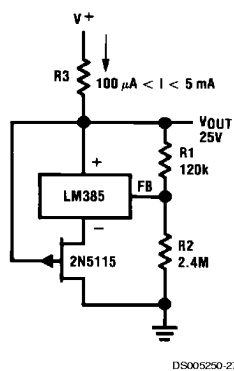
25V Low Current Shunt Regulator
