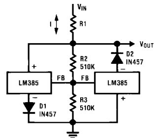
Bidirectional Clamp \pm 2.4V
