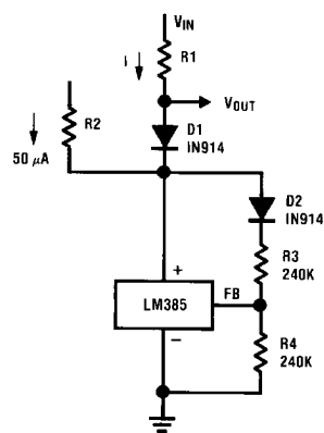
Fast Positive Clamp 2.4V + \Delta V_{D1}
