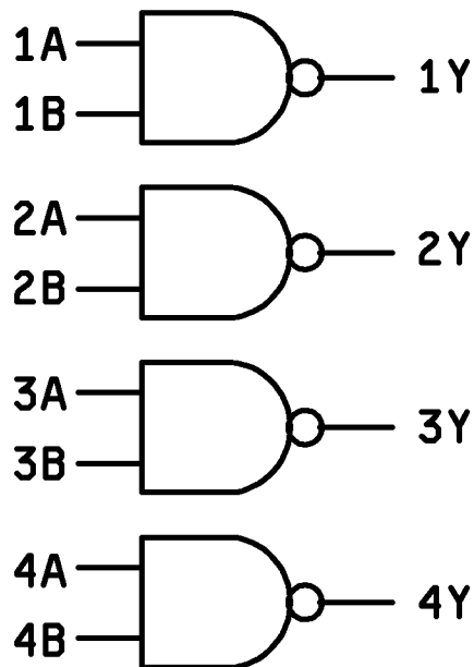
FIGURE 3. Logic diagram.
