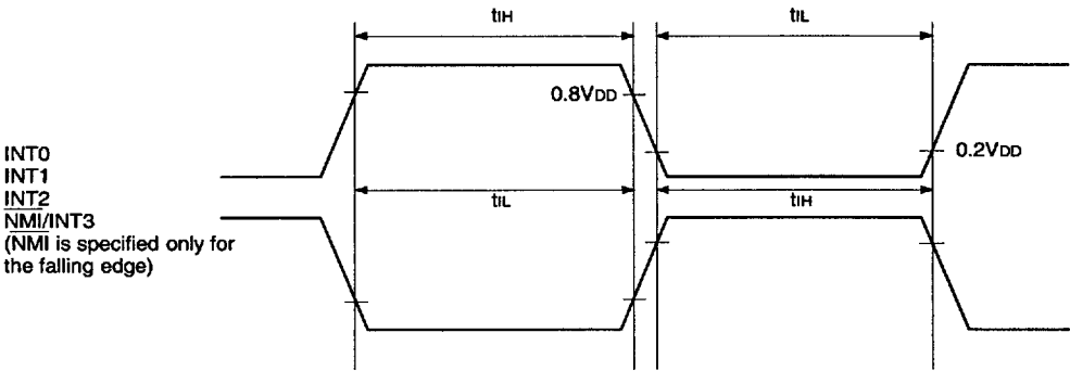
Fig 6. Interruption input timing
