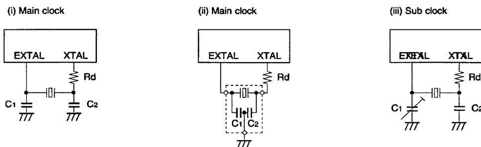
Fig. 8. SPC700 Series recommended oscillation circuit
