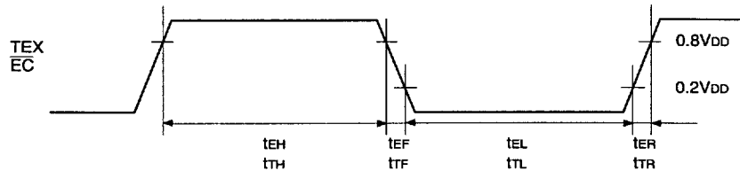
Fig. 3. Event count clock timing
