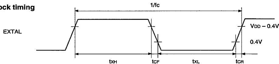
Fig. 2. Clock applied conditions
