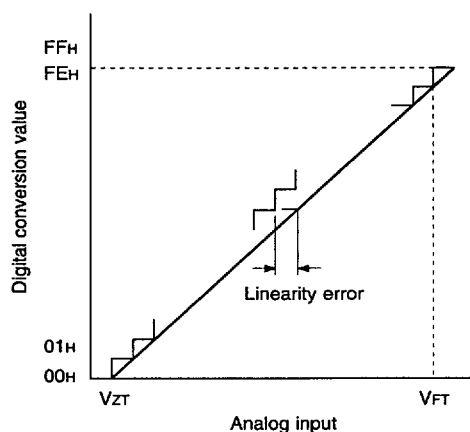
Fig. 5. Definition of A/D converter terms
