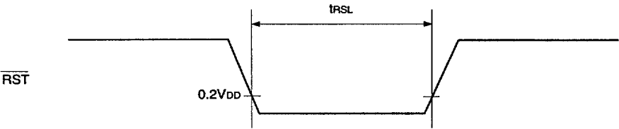
Fig. 7. \overline{\text{RST}} input timing
