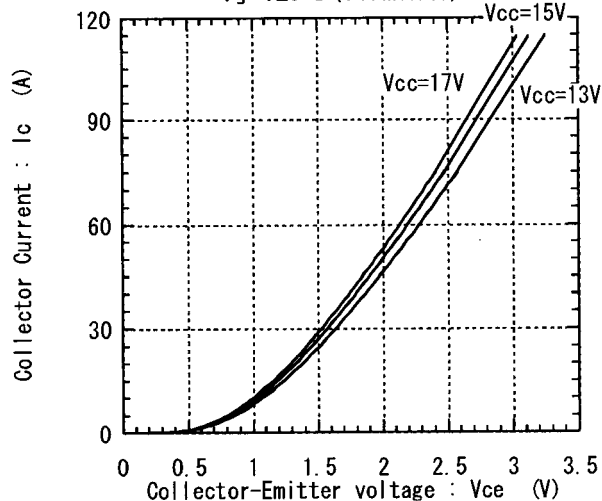
Collector current vs. Collector-Emitter voltage T_j=125^\circ\text{C} (Chip) Collector current vs. Collector-Emitter voltage T_j=125^\circ\text{C} (Terminal)
