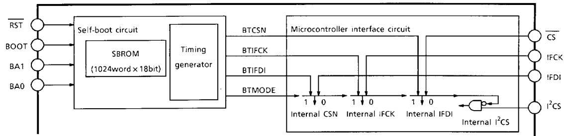
Figure 1 Self-boot system
