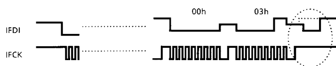
Figure 5 Timing at the time of self boot command transmission
