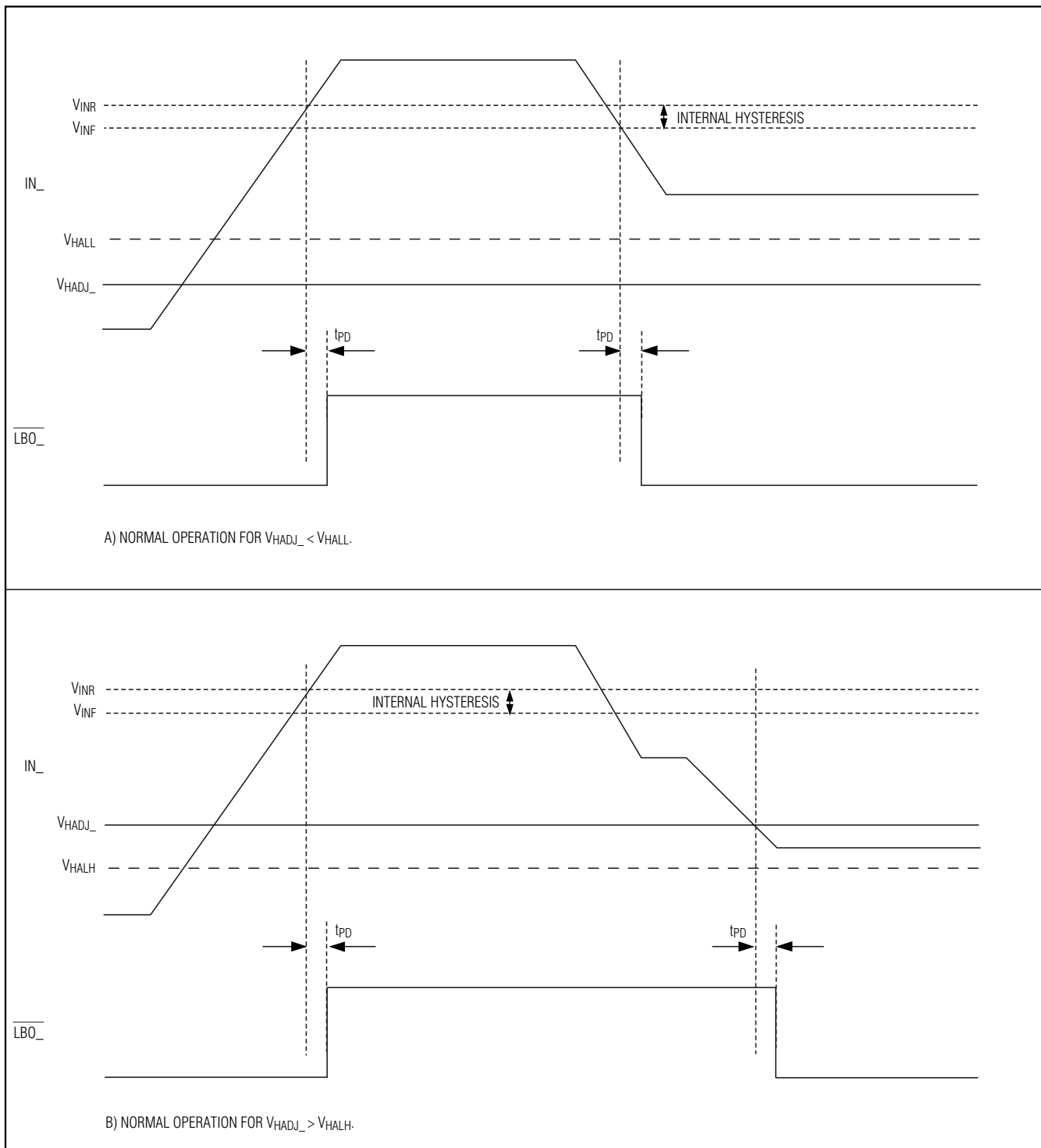
Figure 4. MAX6782-MAX6785 Timing
