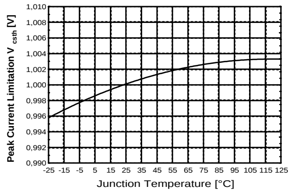
Figure 43 Peak Current Limitation V_{csth} vs. T_j
