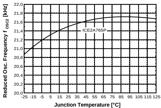
Figure 31 Reduced Osc. Frequency f_{osc2} vs. T_j
