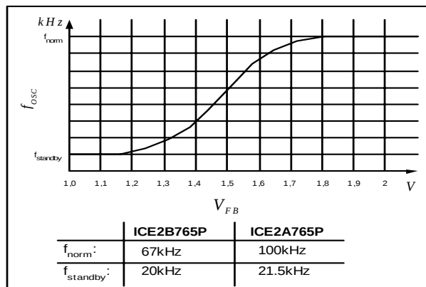
Figure 12 Frequency Dependence
