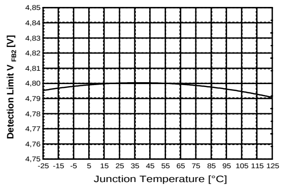
Figure 39 Detection Limit V_{FB2} vs. T_j
