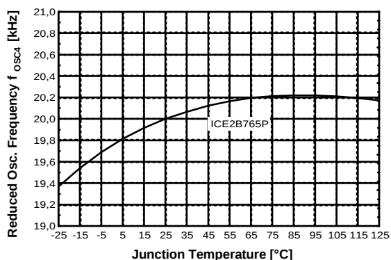
Figure 32 Reduced Osc. Frequency f_{osc4} vs. T_j
