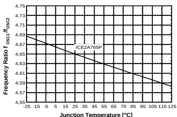
Figure 33 Frequency Ratio f_{osc1} / f_{osc2} vs. T_j
