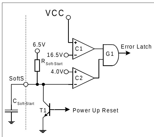
Figure 21 Overvoltage Detection
