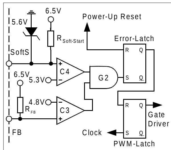
Figure 10 Activation of Protection Unit
