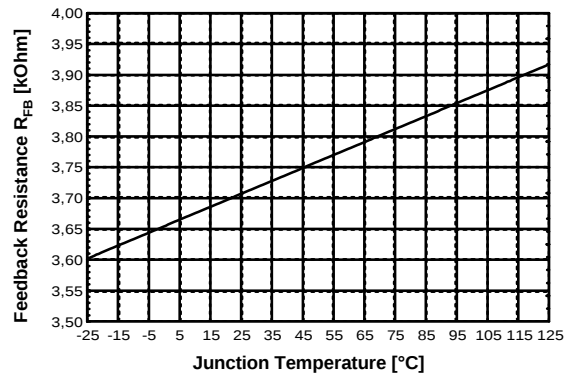
Figure 37 Feedback Resistance R_{FB} vs. T_j
