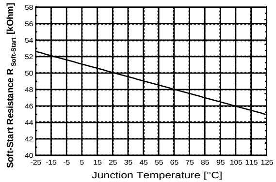
Figure 38 Soft-Start Resistance R_{Soft-Start} vs. T_j
