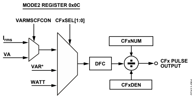
Figure 79. Energy-to-Frequency Conversion
