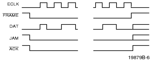
Figure 2. Asynchronous Mode Data Transfer
