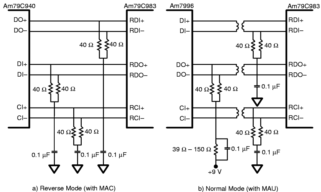
Figure 9. RAUI Port Interconnections
