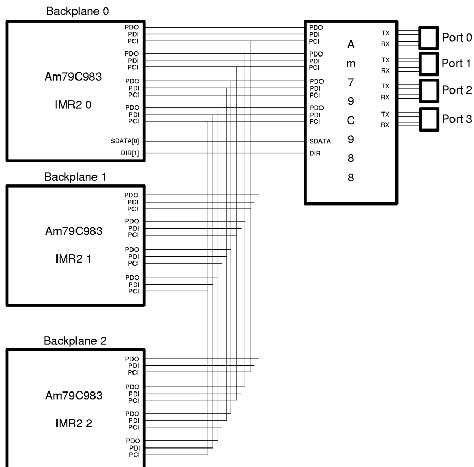
Figure 11. Port Switching Configuration
