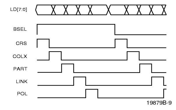
Figure 5. Visual Monitor Signals
