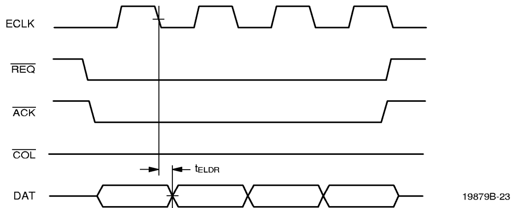
Figure 19. Expansion Port Output Timing - Asynchronous Mode
