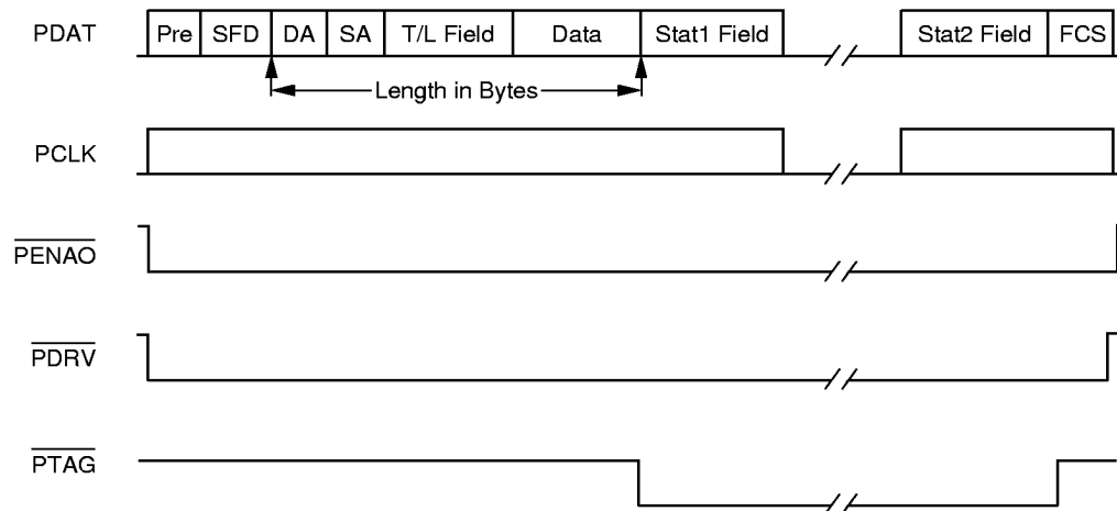
Figure 4. Packet Port Signals
