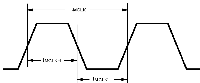
Figure 12. Master Clock (MCLK) Timing
