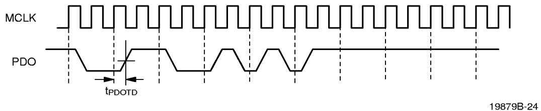
Figure 20. PAUI PDO Transmit
