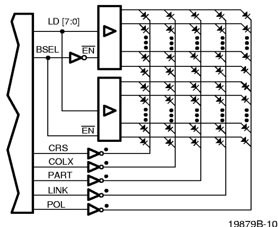
Figure 6. Visual Monitoring Application - Simplified Schematic
