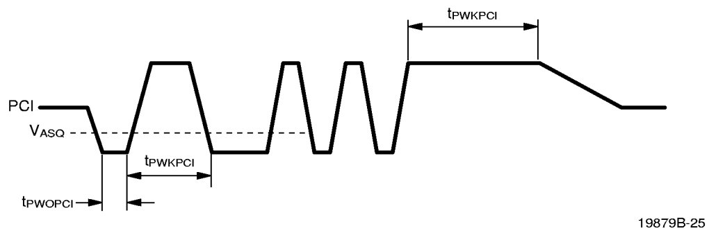
Figure 21. PAUI PCI Receive
