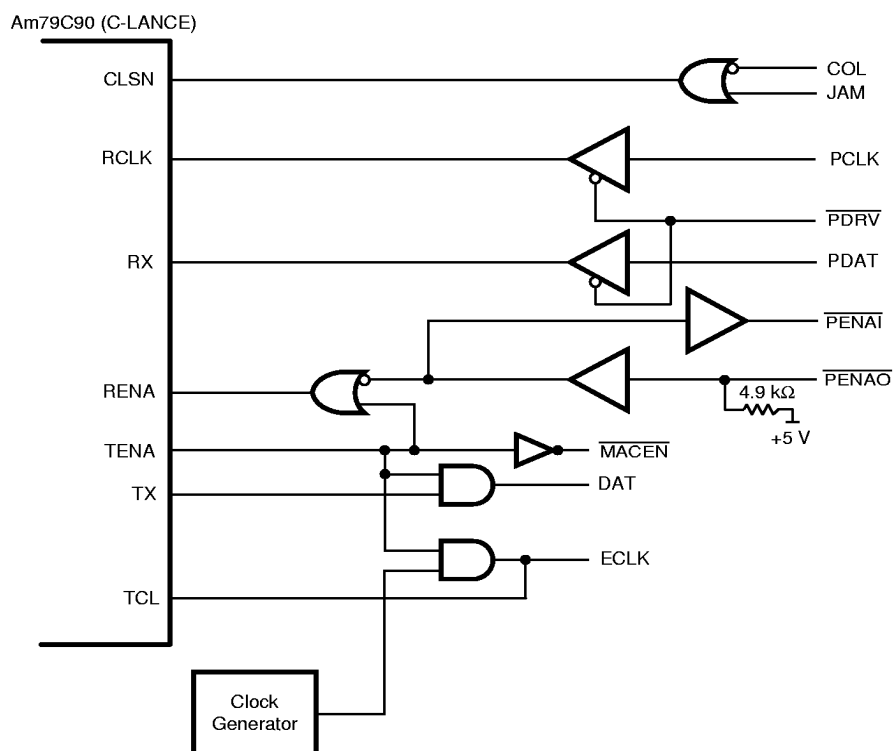
Figure 10. PR Port Connection to an Am79C90 C-Lance
