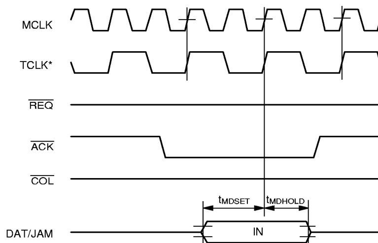
Figure 14. Expansion Bus Input Timing - Synchronous Mode
