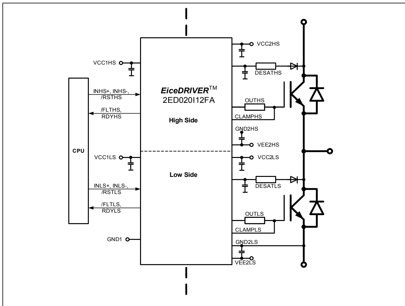
Figure 1: Typical Application
