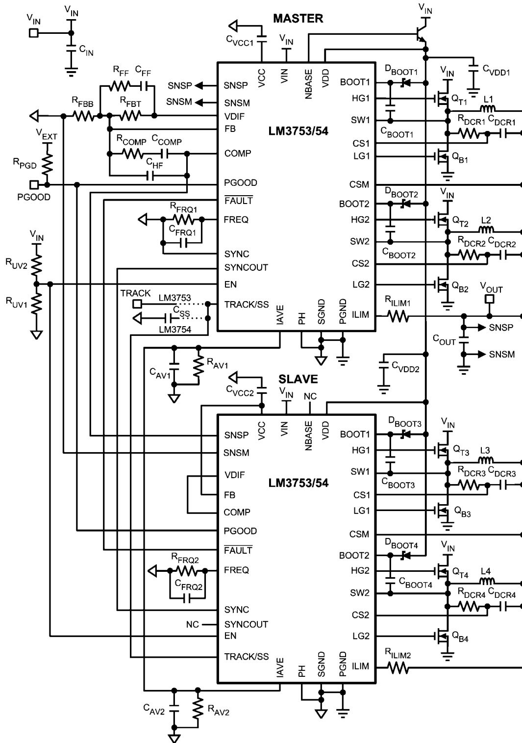
FIGURE 20. Typical Application
