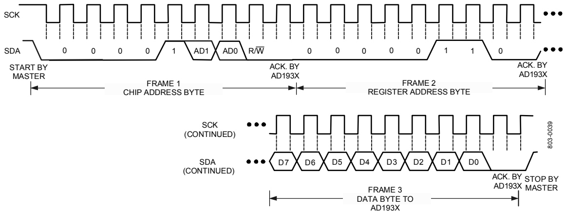
Figure 11. Format of I 2 C Write
