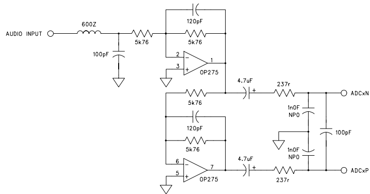
Figure 23. Typical ADC Input Filter Circuit
