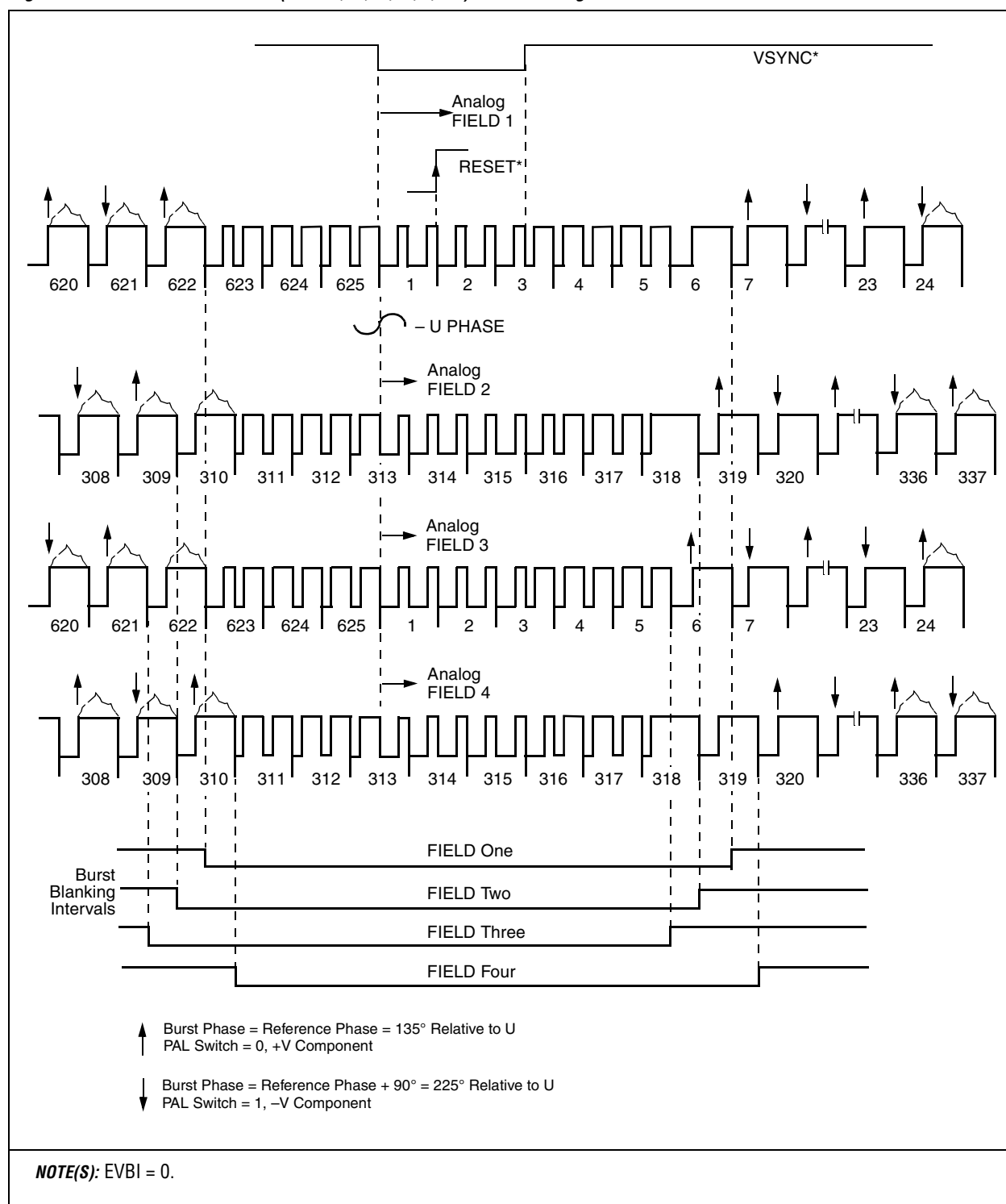
Figure 1-6. Interlaced 625-Line (PAL-B, D, G, H, I, Nc) Video Timing
