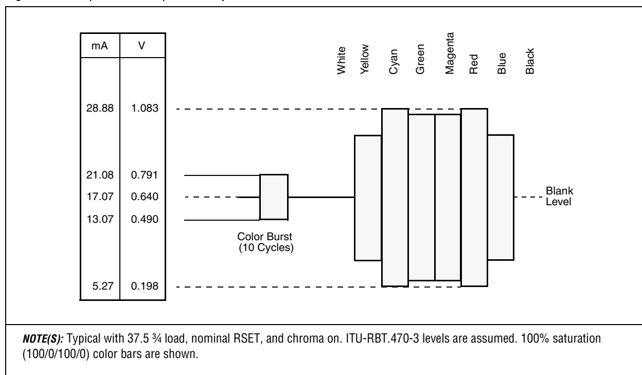
Figure 1-25. C (Chrominance) Video Output Waveform SETUPDIS = 1
