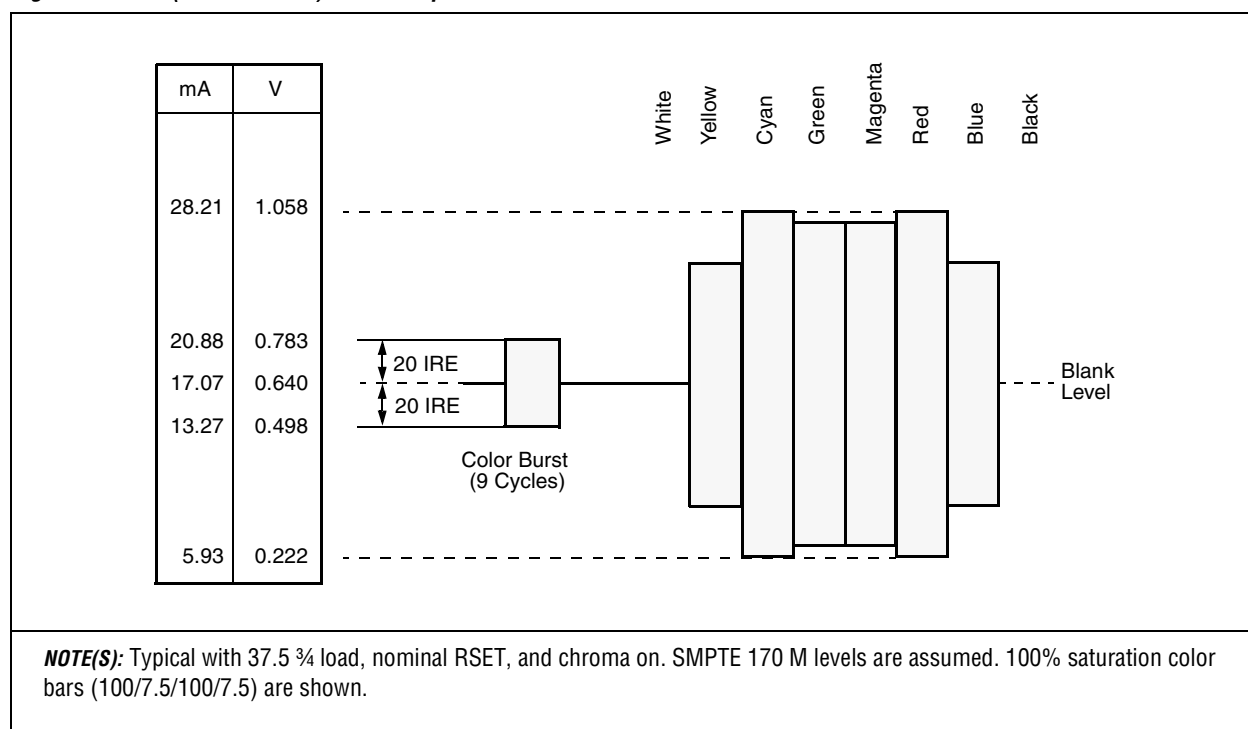
Figure 1-24. C (Chrominance) Video Output Waveform SETUPDIS = 0
