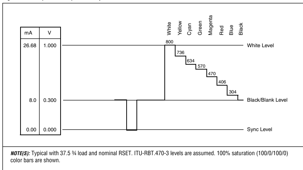
Figure 1-23. Y (Luminance) Video Output Waveform SETUPDIS = 1
