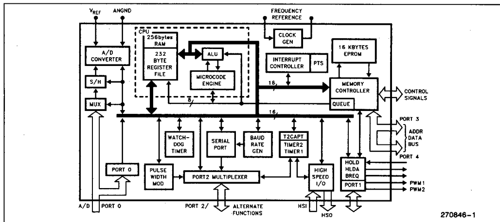
Figure 1. 87C196KC Block Diagram
