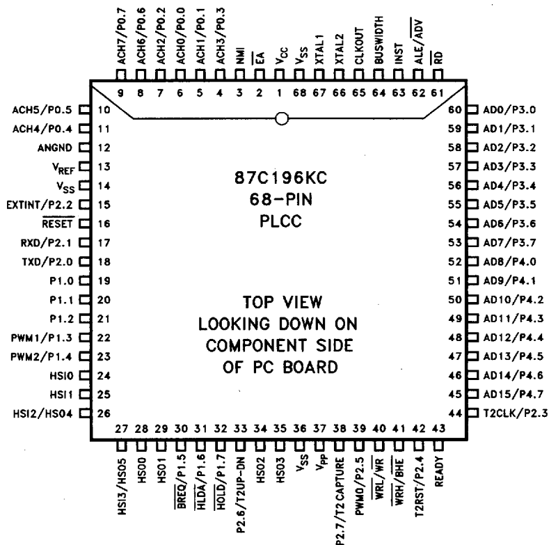
Figure 4. 68-Pin PLCC Package
