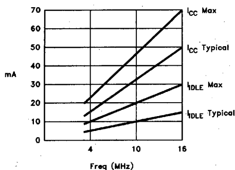
Figure 5. I_{CC} and I_{IDLE} vs Frequency
