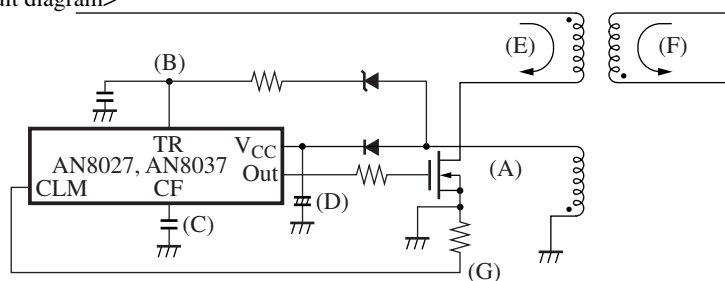
<Circuit diagram>
