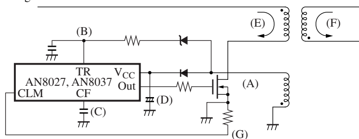
<Circuit diagram>
