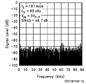
Spectral Response with 90 KHz Sine Wave Input
