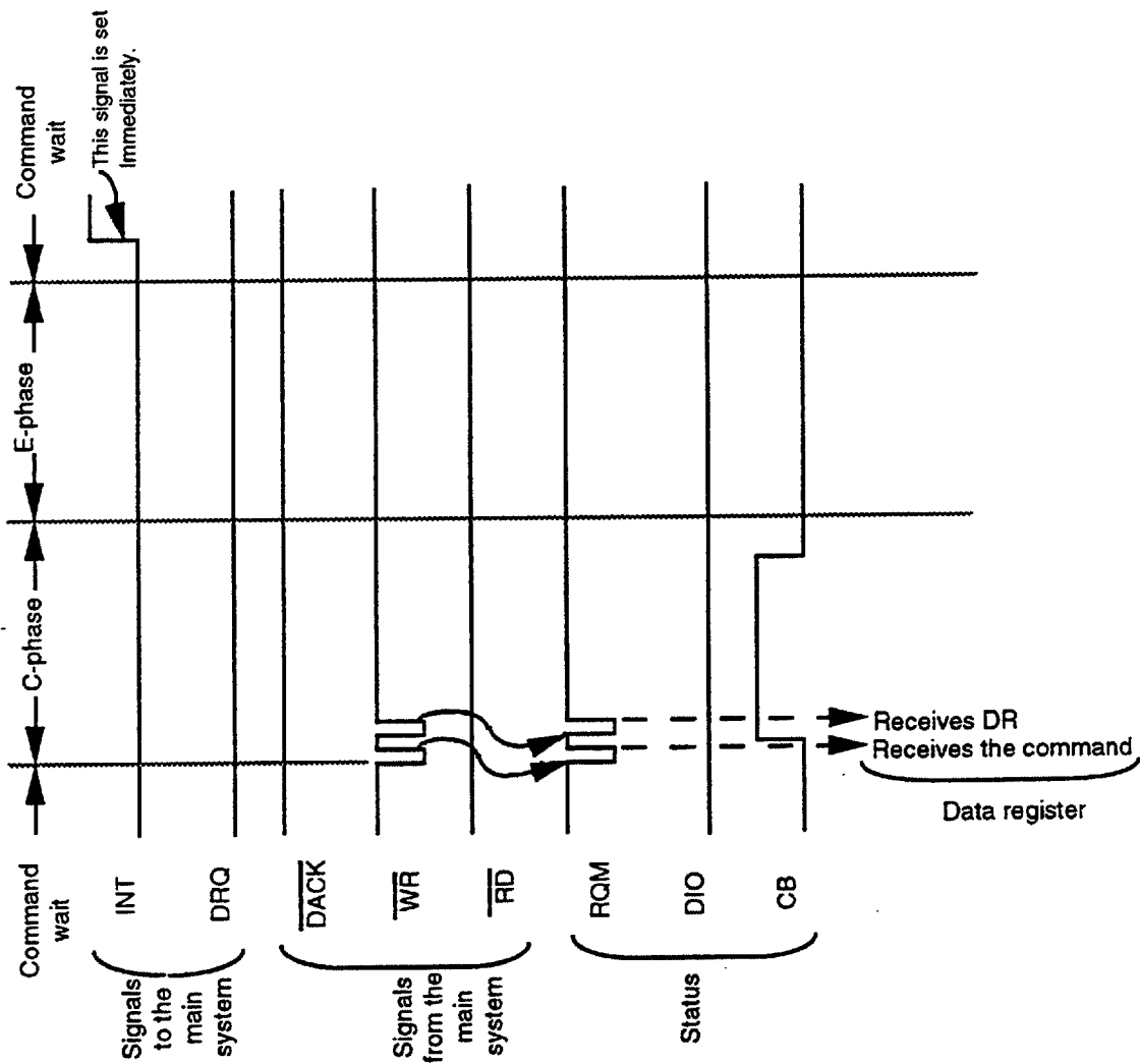
Fig.5.1-9 EJECT DISK command
