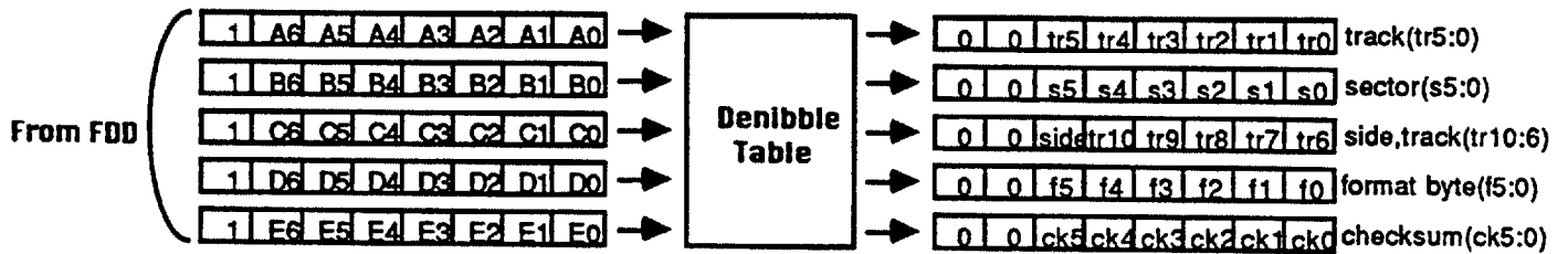
Fig. 1.3.7 Address Header Denibblizing Process
