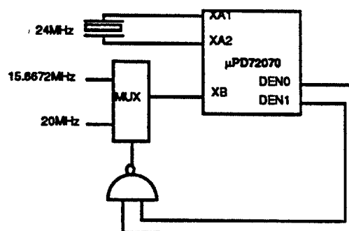
Recommended Circuit #2
