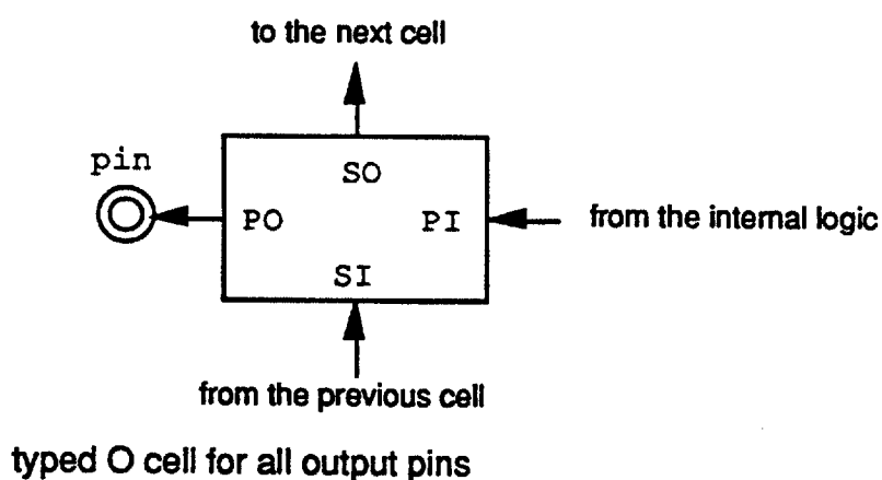
Fig 8.4.3.1 the O typed cells
