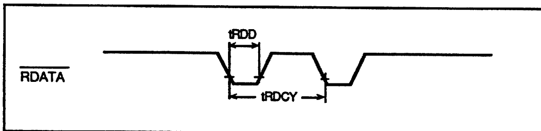
Fig.7 MFM FDD Read Data Timing
