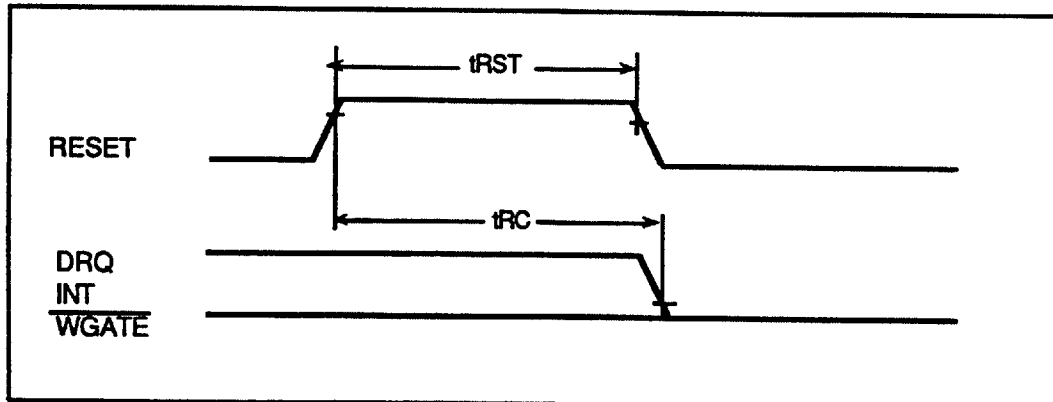
Fig.5 Reset Timing
