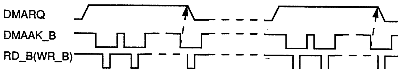
Single Transfer Mode
