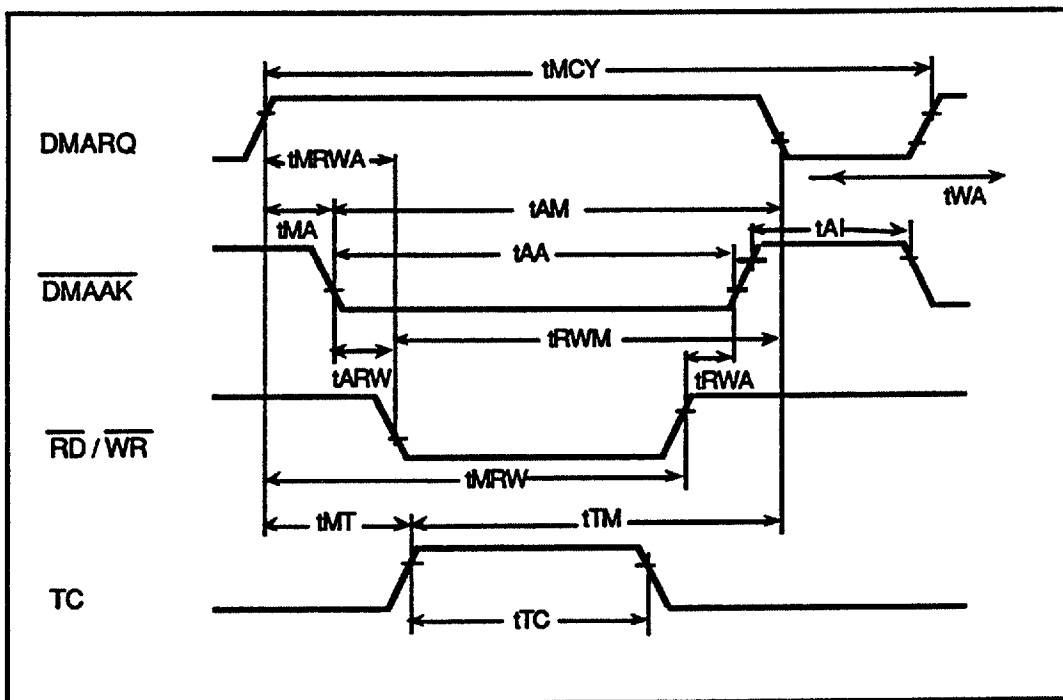
Fig.4 DMA Timing
