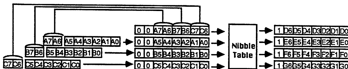
Fig. 1.3.4 Nibblizing process for Sector Data
