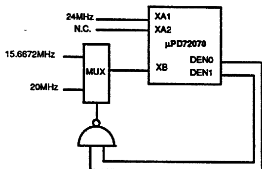
Crystal Clock Oscillators
