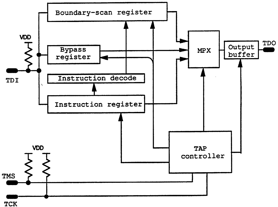
Fig 8.2 A Block Schematic of the Test Logic
