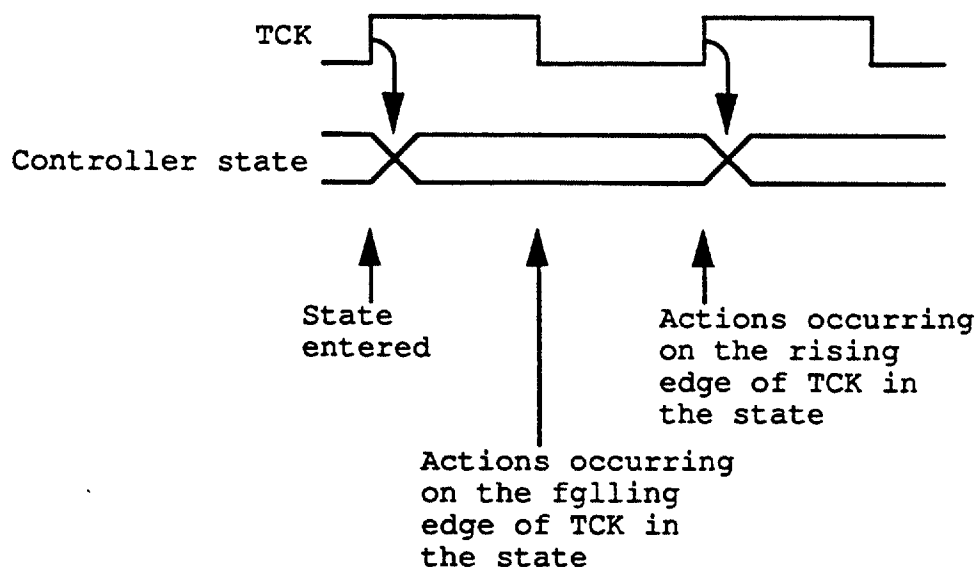
Fig 8.4-2 TAP Controller State Diagram
