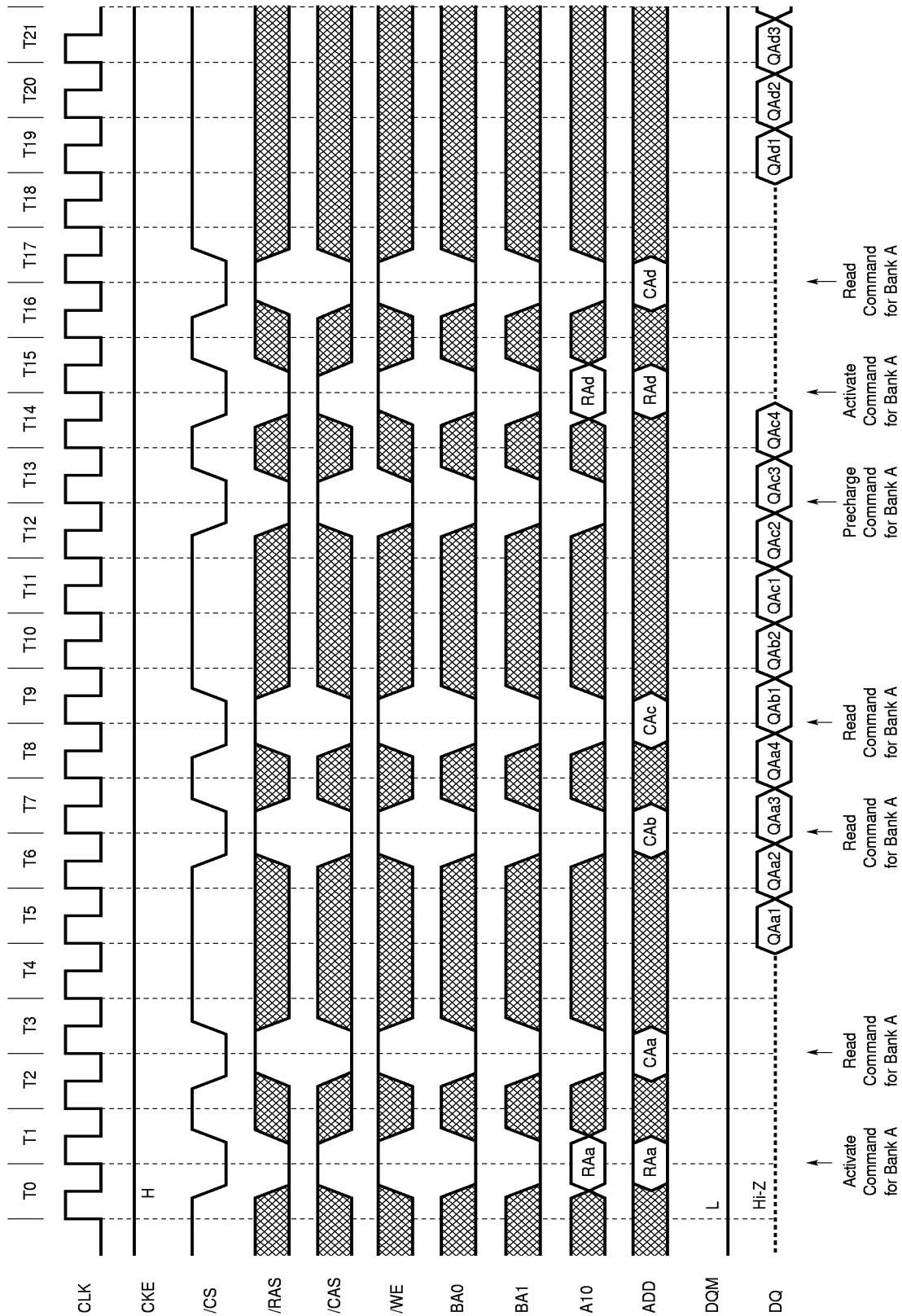
13.12 Random Column Read (Page with Same Bank) (1/2) (Burst Length = 4, /CAS Latency = 2)
