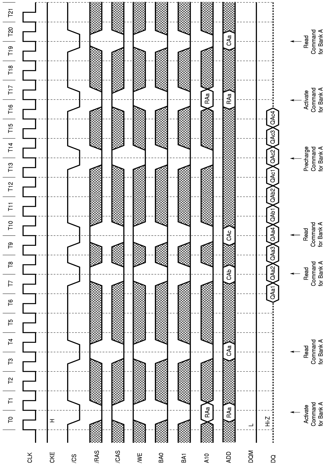
Random Column Read (Page with Same Bank) (2/2) (Burst Length = 4, /CAS Latency = 3)
