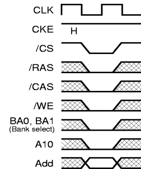
Fig.2 Row address strobe and bank activate command
