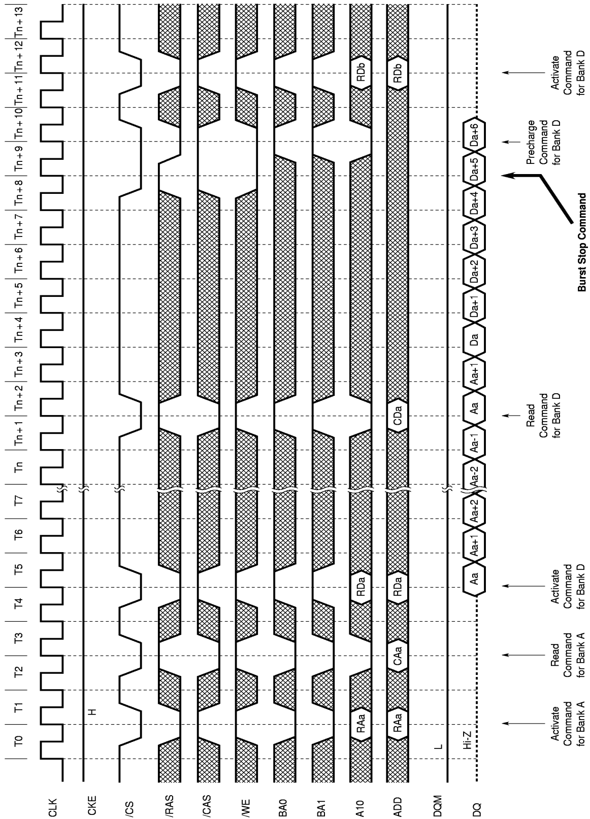
13.21 Full Page Read Cycle (1/2) (/CAS Latency = 2)
