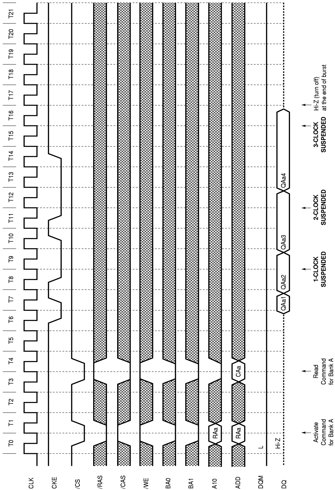
Clock Suspension during Burst Read (using CKE Function) (2/2) (Burst Length = 4, /CAS Latency = 3)
