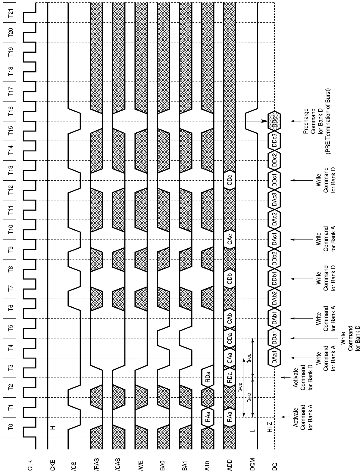
13.26 Full Page Random Column Write (Burst Length = Full Page, /CAS Latency = 2)
