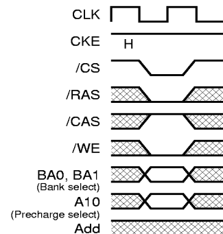
Fig.3 Precharge command
