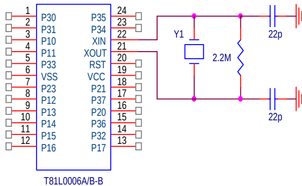
Crystal Oscillator
