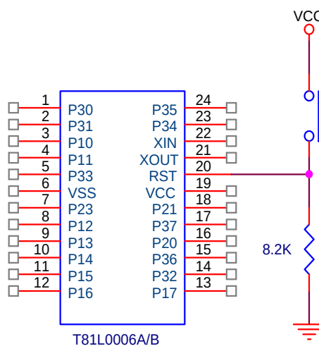
For Power on Reset and External Reset
