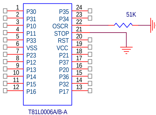
RC Oscillator
