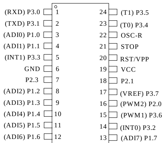
DIP-24/SOP-24 For RC Oscillator T81L0006A-AK/ T81L0006A-AD T81L0006B-AK/ T81L0006B-AD
